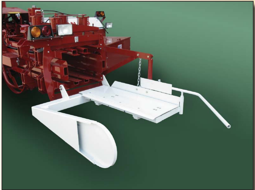
Digital Bale Scale (Allied Systems Company Part #905895) Shown Mounted on a Freeman 370 Baler
