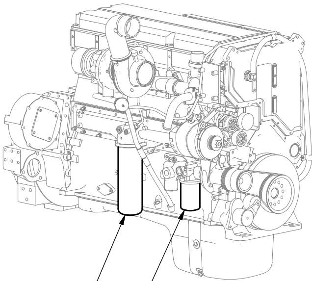
Oil Filter 588563
