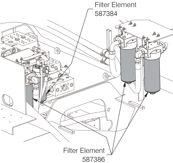
High Pressure Hydraulic Filters Access from Deck, Under Boom
