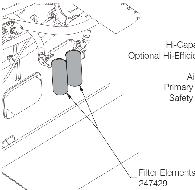
Transmission Filters Access from Under Chassis, Left Side
