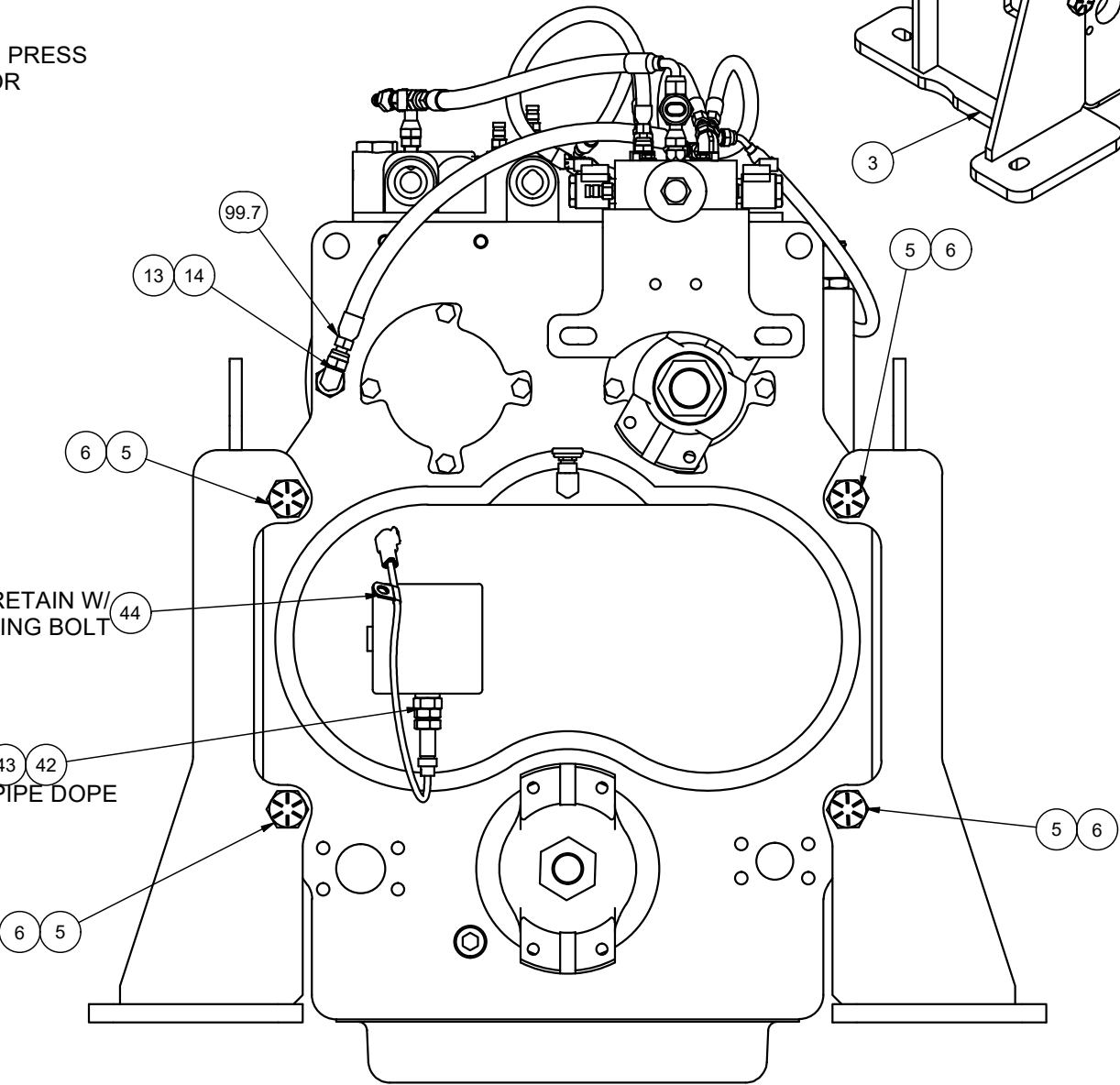
BACK VIEW
