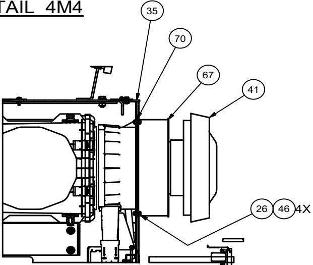
DETAIL 4M4
