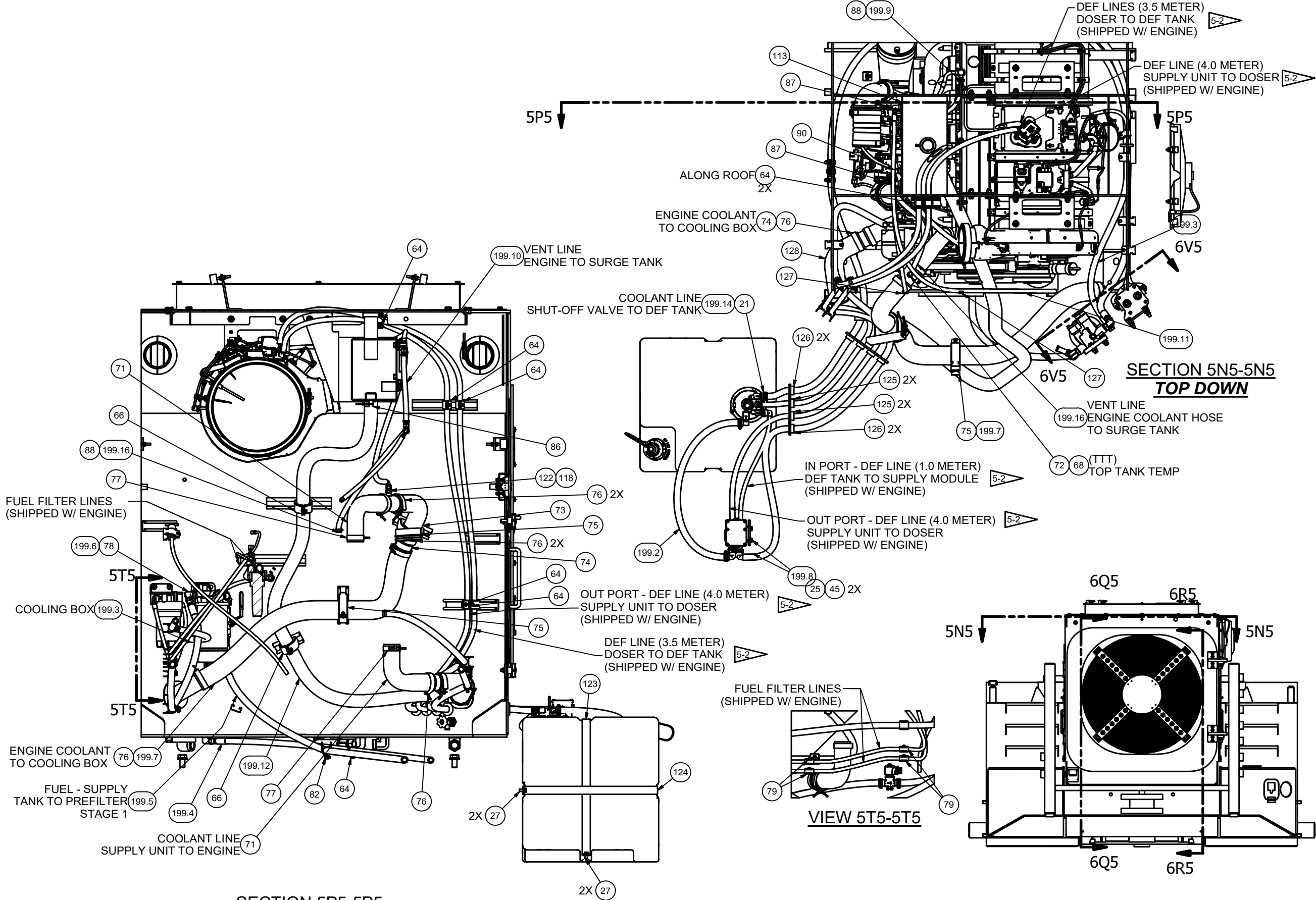
SECTION 5P5-5P5 VIEW ROTATED BACK OF COOLING BOX
