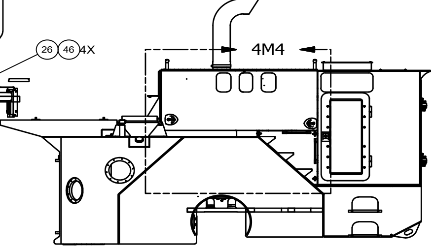
SECTION 4L4-4L4
