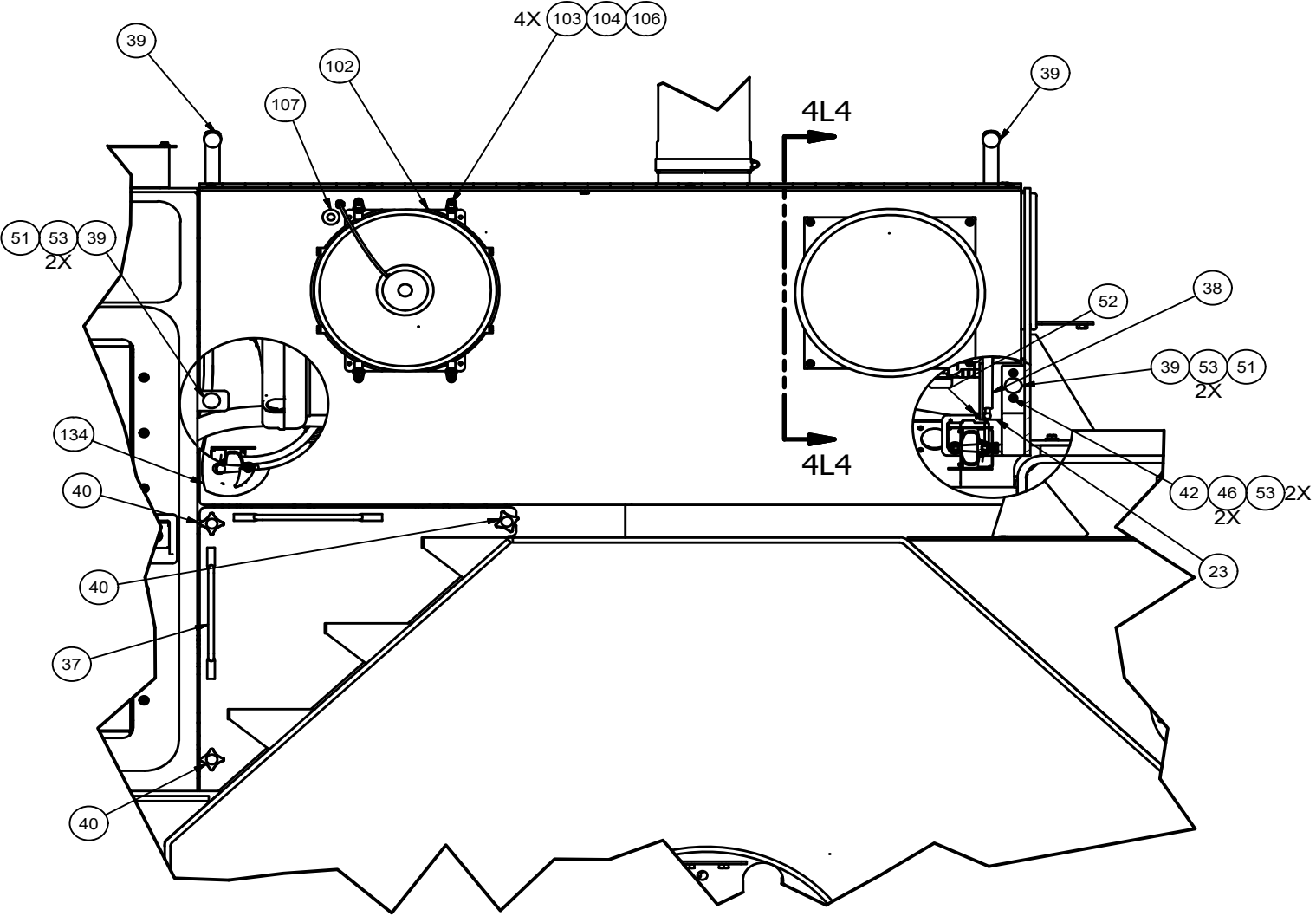
DETAIL 4K4
