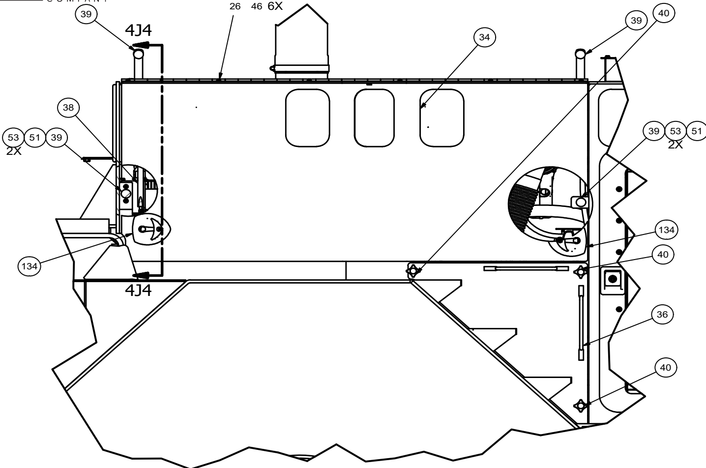
DETAIL 4M4
