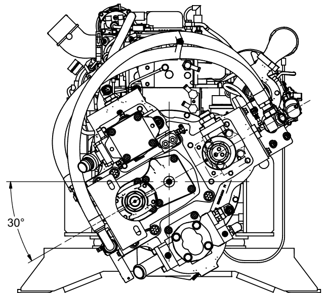
BACK VIEW ORIENT CONV. AS SHOWN
