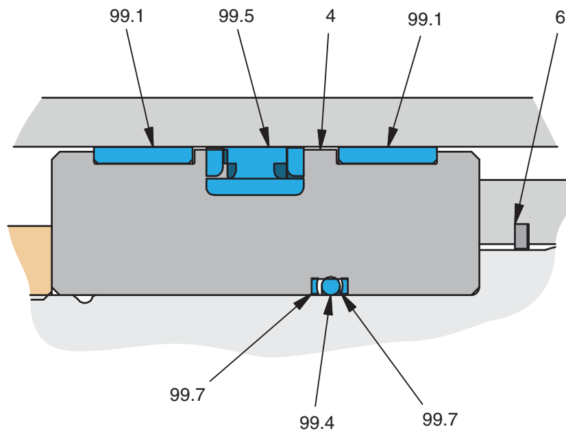
Detail at Piston
