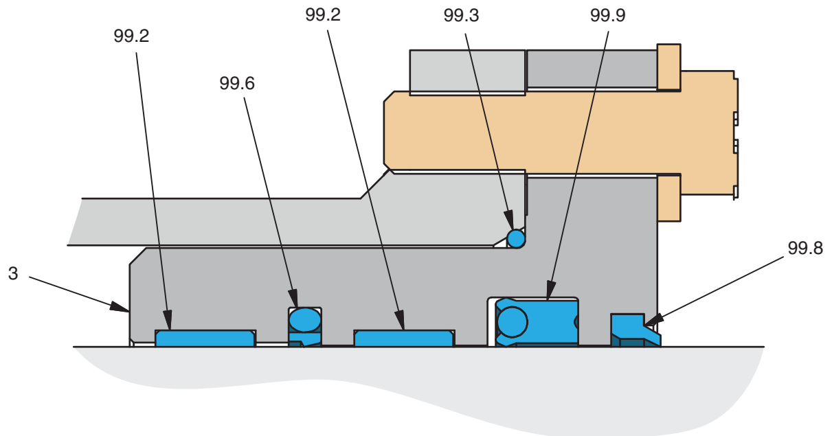
Detail at Packing Gland
