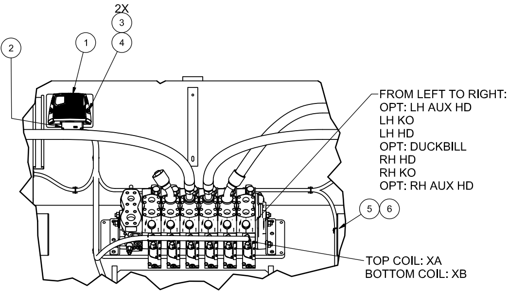
DETAIL 15BD15 SOME PARTS REMOVED FOR CLARITY
