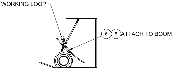
SECTION 15BF15-15BF15 BOOM-CARRIAGE POSITION SENSOR
