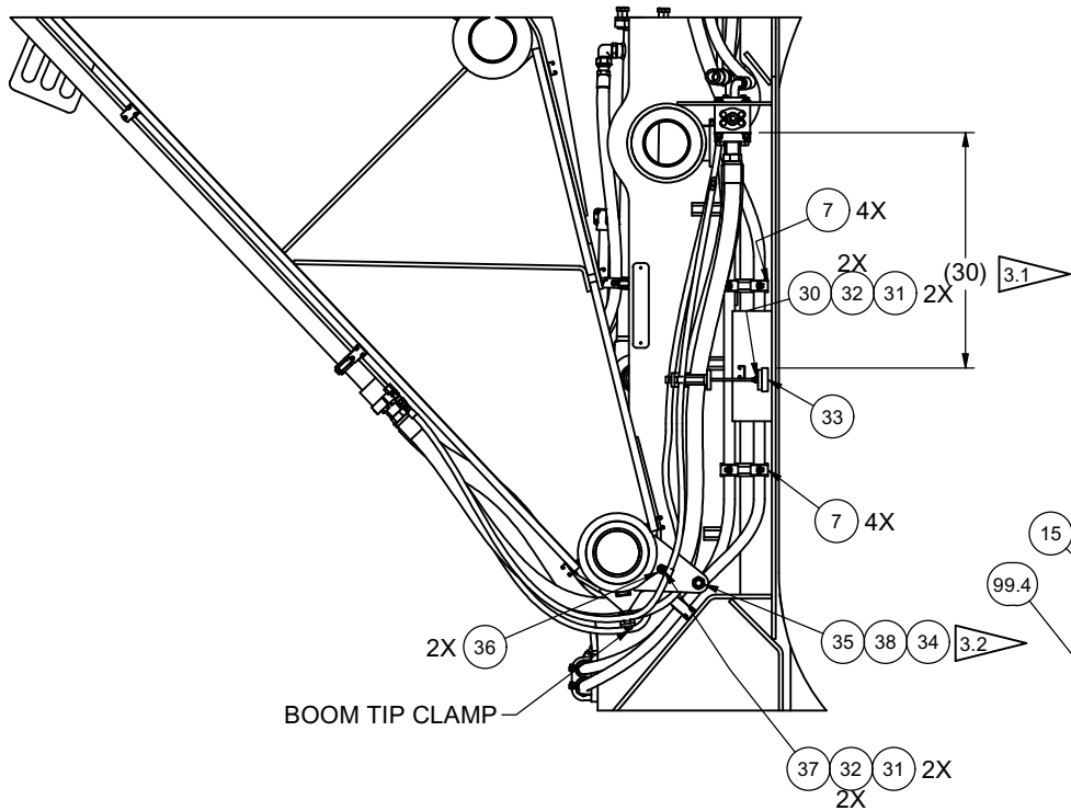
SECTION 3E2-3E2 VIEW CROPPED FOR CLARITY
