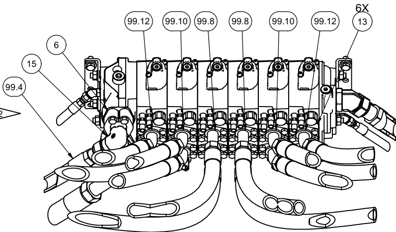
TOP OF IMPLEMENT VALVE CARRIAGE WELDMENT REMOVED FOR CLARITY
