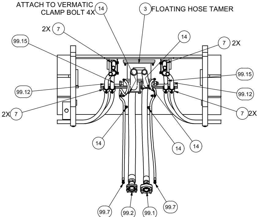
SECTION 3D2-3D2 CARRIAGE WORKING LOOP
