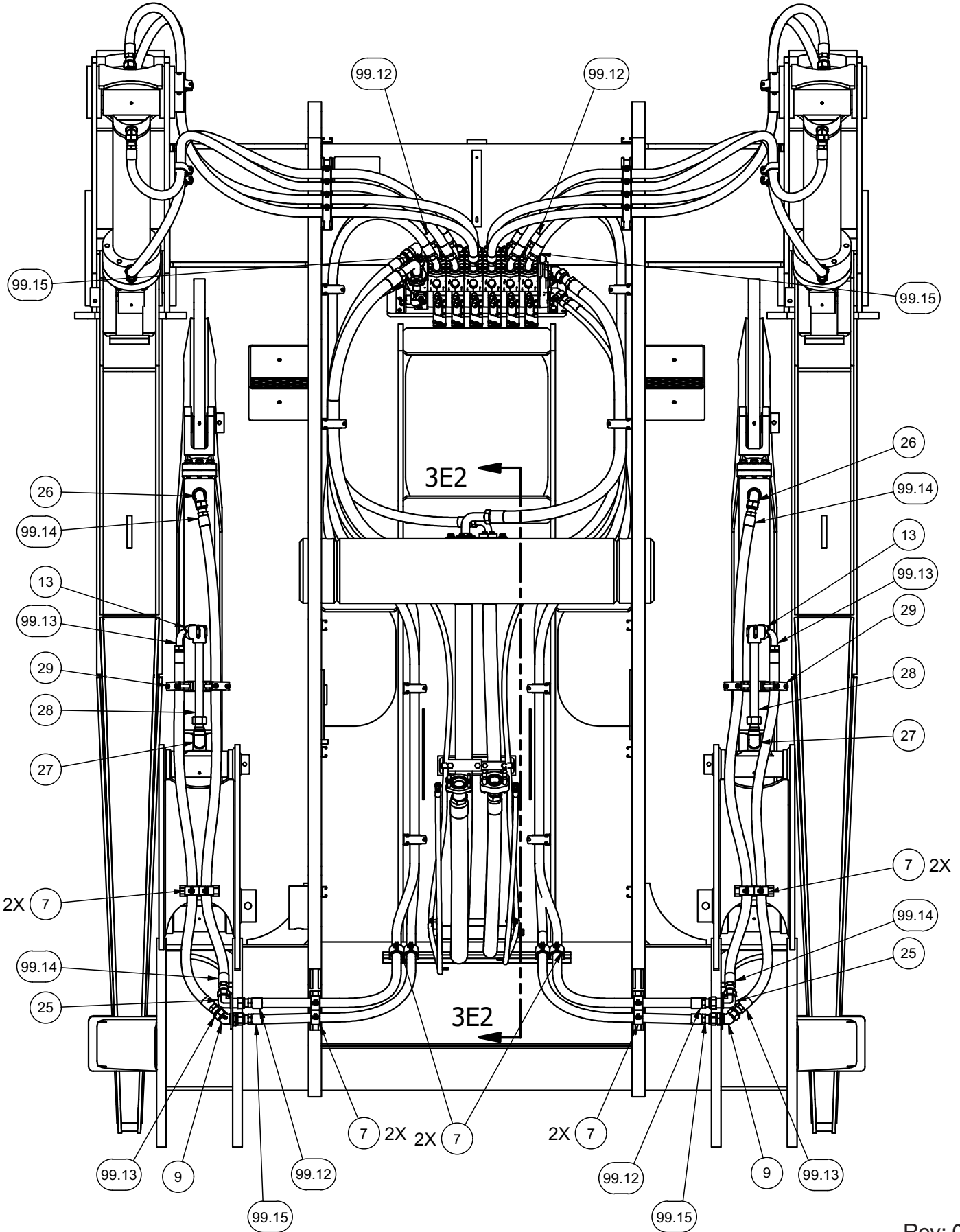
LOW MOUNT AUX HD PLUMBING
