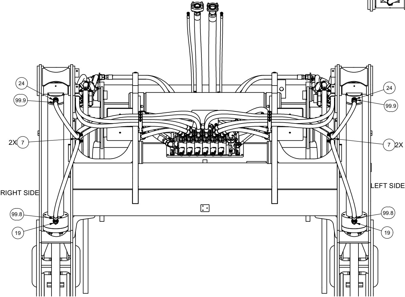
TOP VIEW HD CYLINDER PLUMBING
