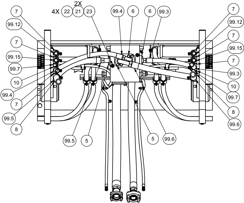
SECTION 4B2-4B2 CARRIAGE DISTRIBUTION MANIFOLD SOME PARTS REMOVED FOR CLARITY
