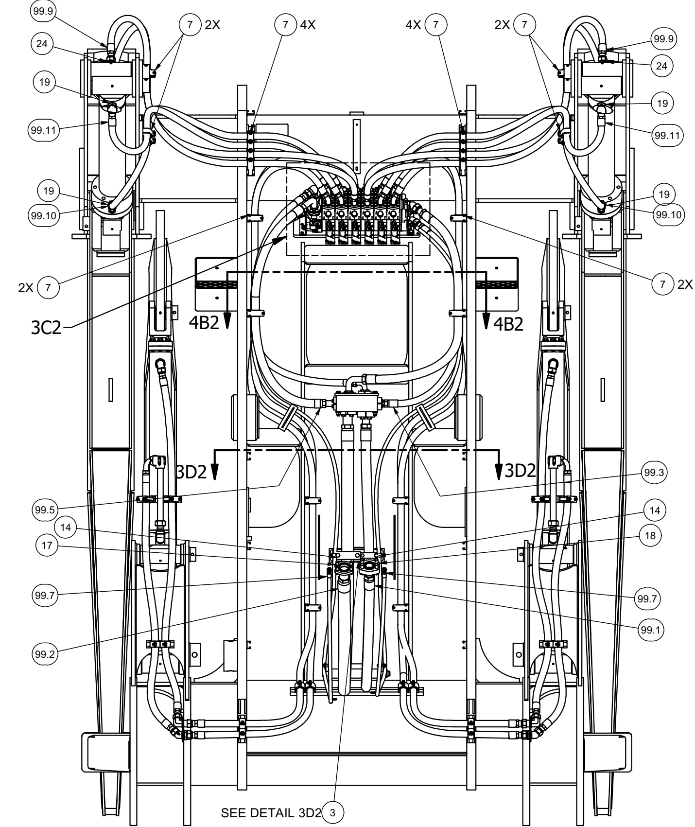
VIEW 2A1-2A1 SOME PARTS REMOVED FOR CLARITY
