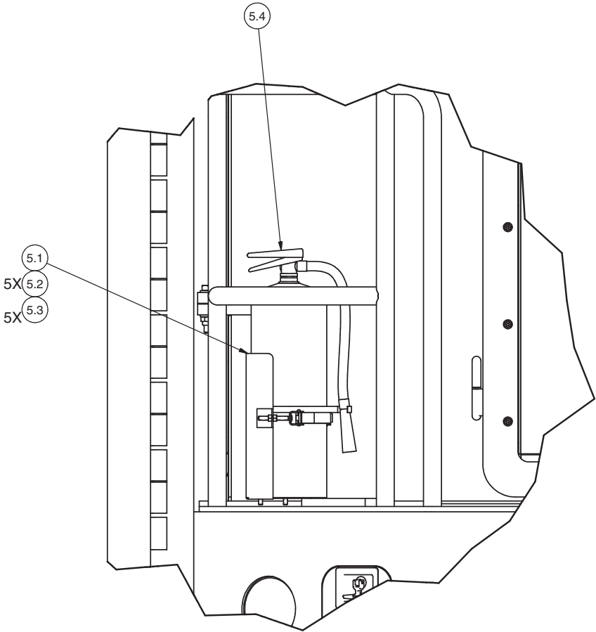
DETAIL 4J4
