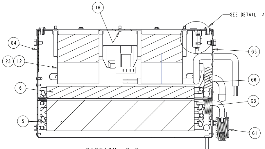
SECTION B-B
