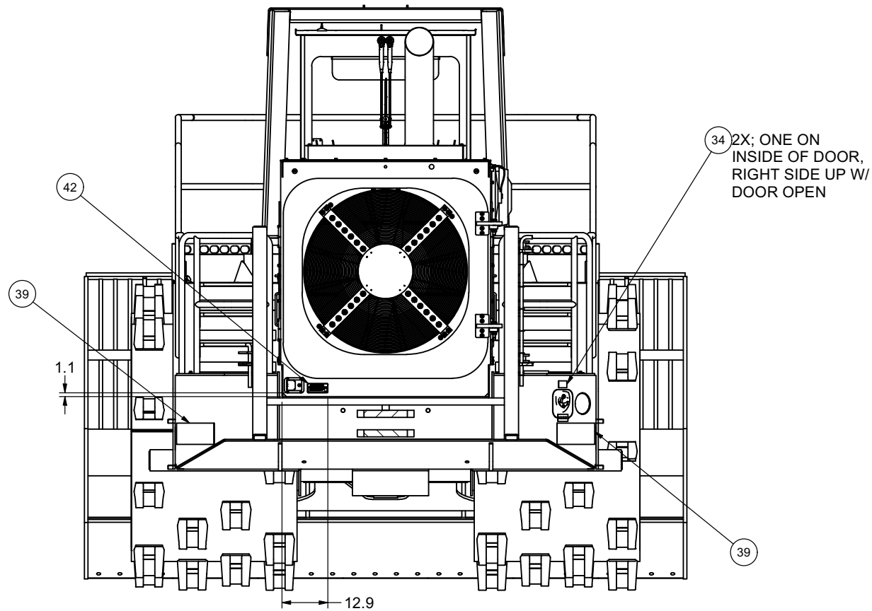
SECTION 2B2-2B2
