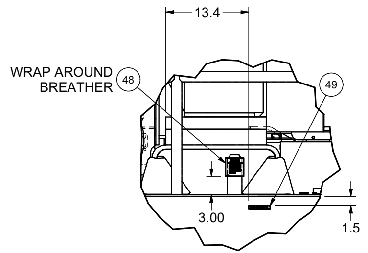
DETAIL 3F3 PARTS HIDDEN FOR CLARITY
