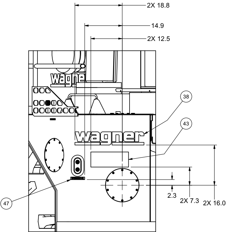
DETAIL 5N4
