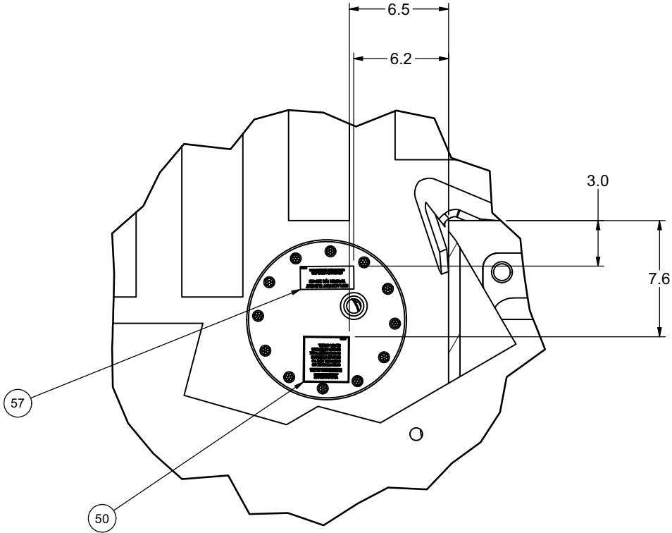
DETAIL 5N4
