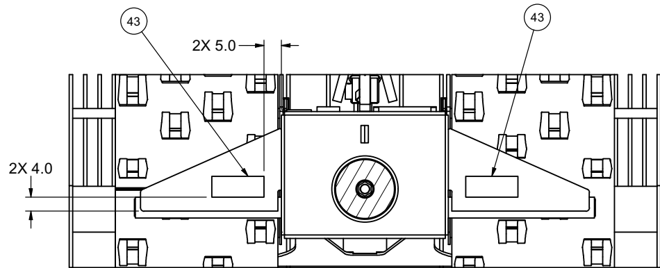
SECTION 2A2-2A2
