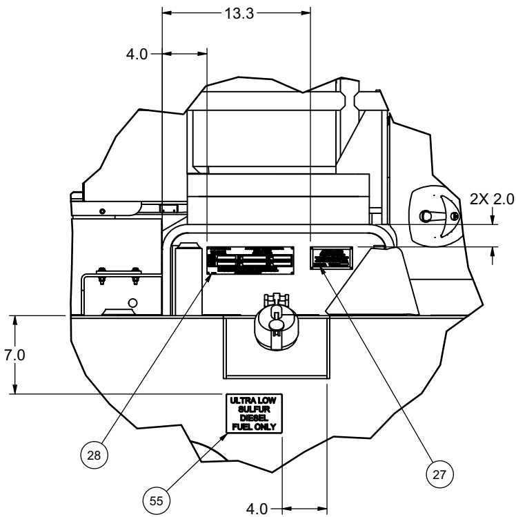
DETAIL 5M2 ITEMS HIDDEN FOR CLARITY
