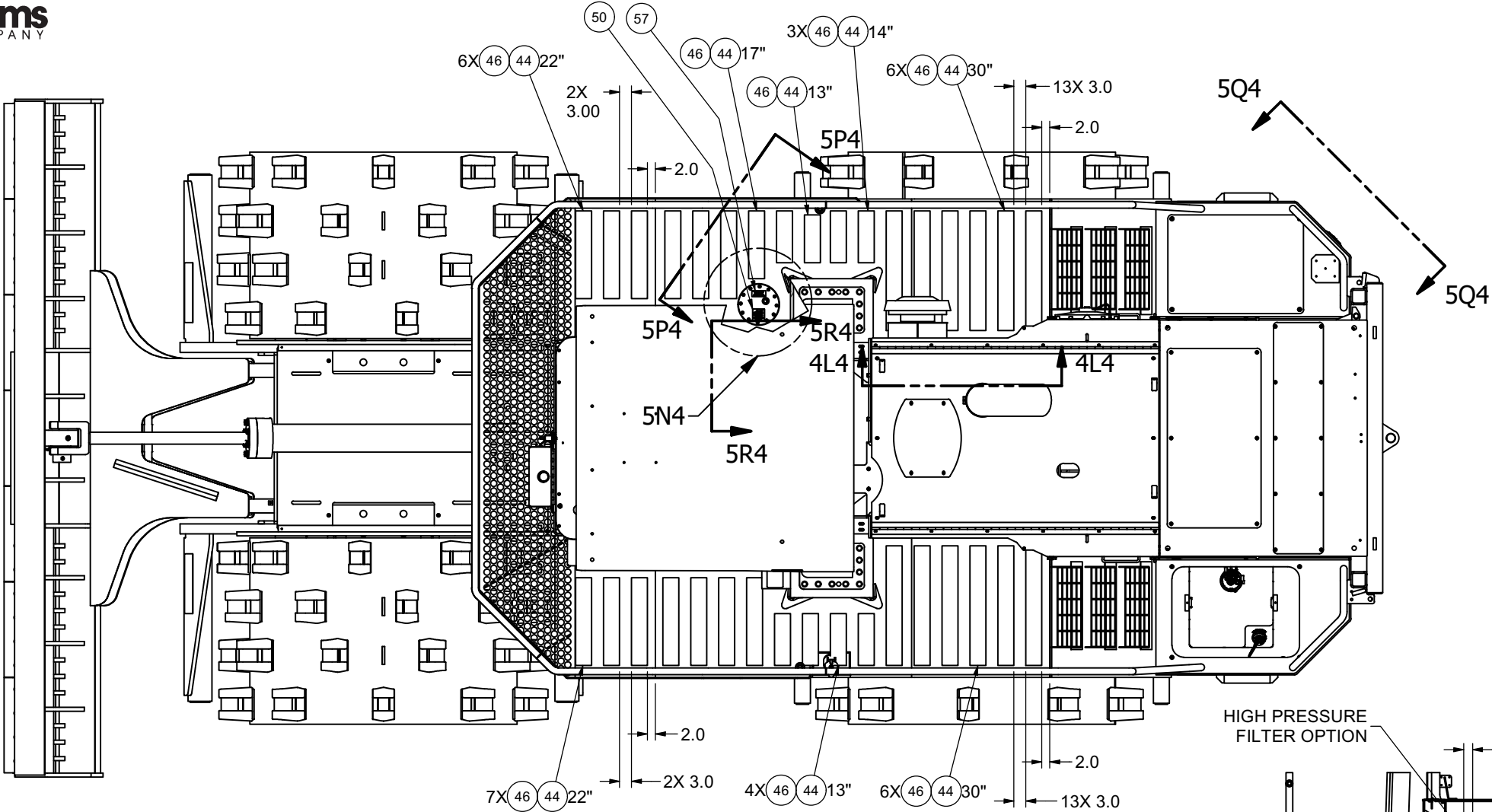
VIEW 4G2-4G2
