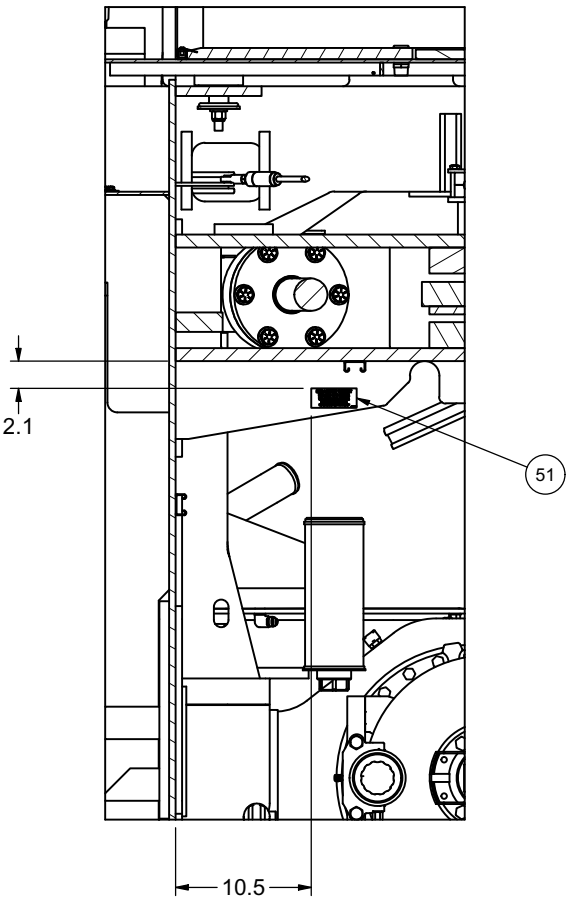
SECTION 5R4-5R4 VIEW CROPPED FOR BETTER CLARITY
