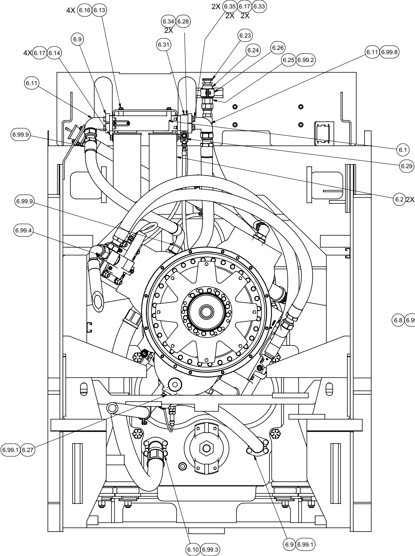
SECTION 11Y10-11Y10 VIEW FROM BACK
