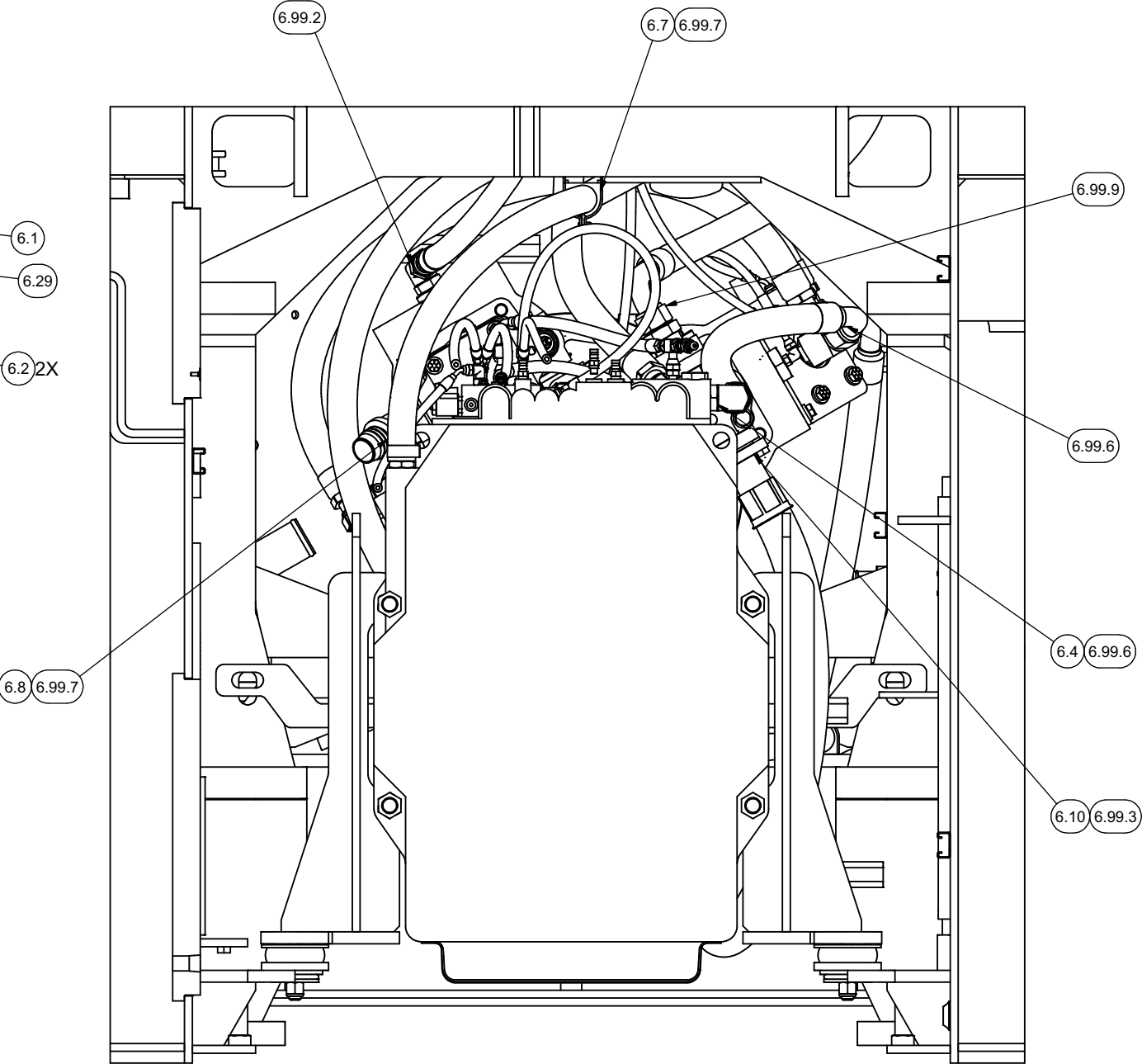
SECTION 11Z10-11Z10 VIEW FROM FRONT
