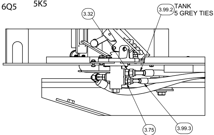
SECTION 5AB5-5AB5
