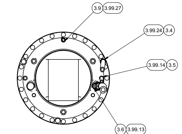
SECTION 5K5-5K5 LH BRAKE HUB PLUMBING
