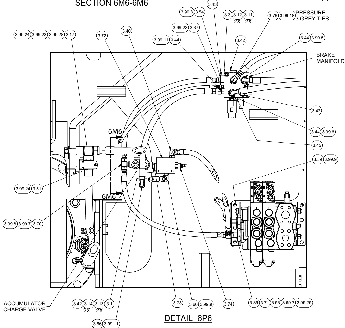
SECTION 6M6-6M6
