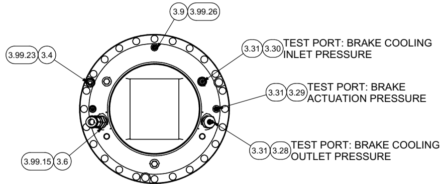
SECTION 5L5-5L5 RH BRAKE HUB PLUMBING
