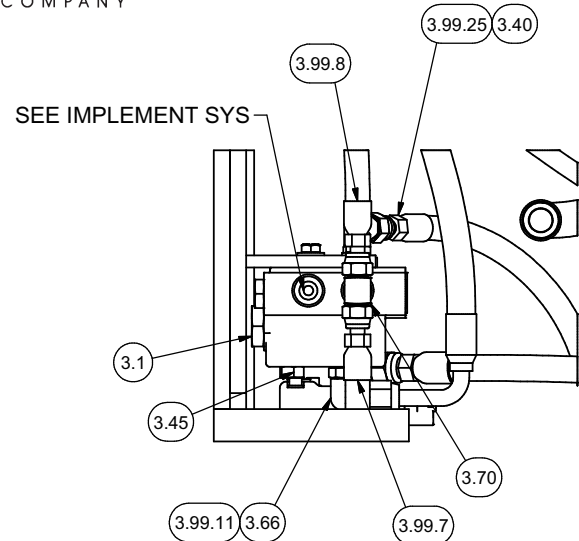
SECTION 6M6-6M6
