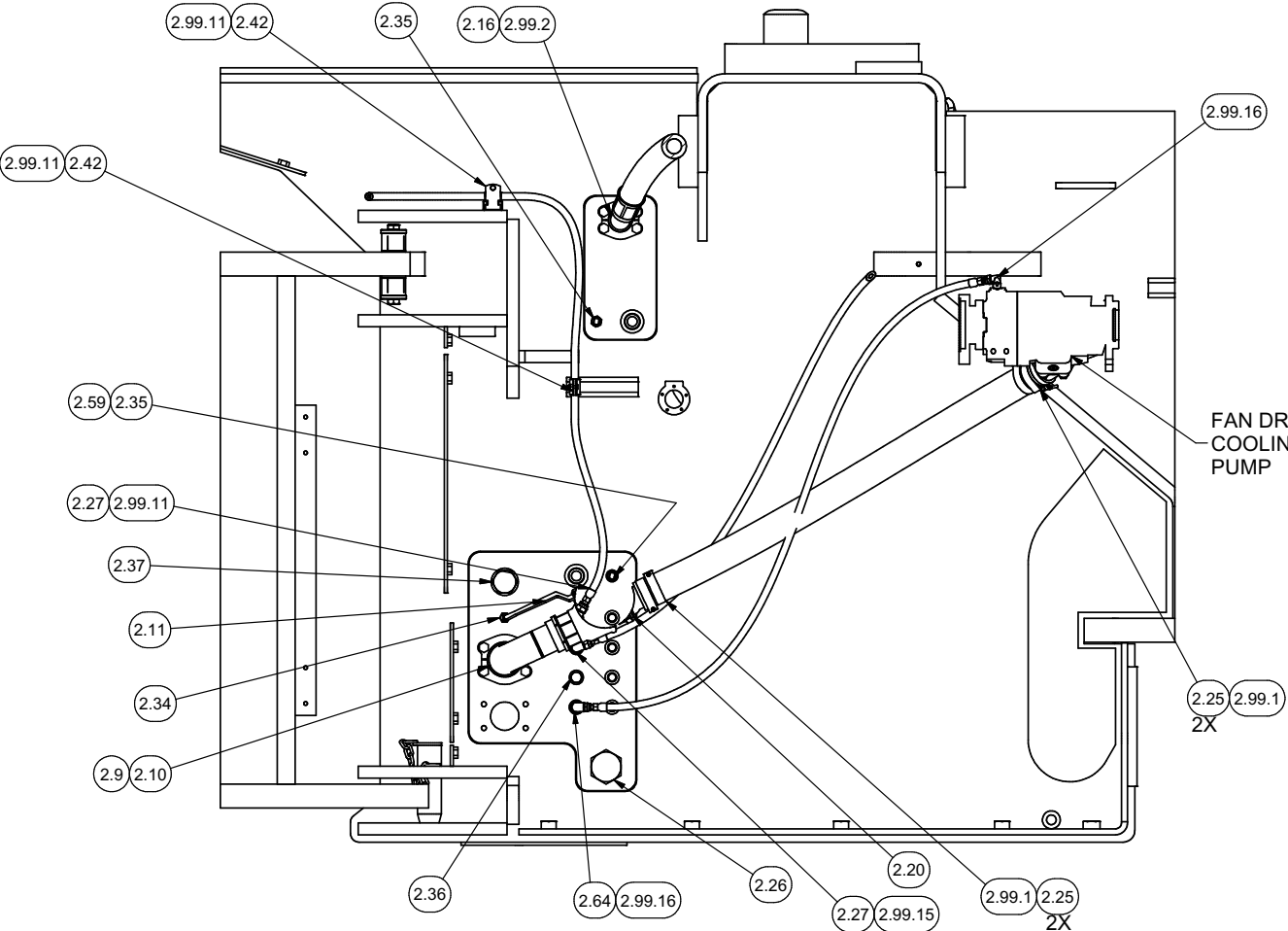
SECTION 4F3-4F3 RH SIDE - NO CYLINDER
