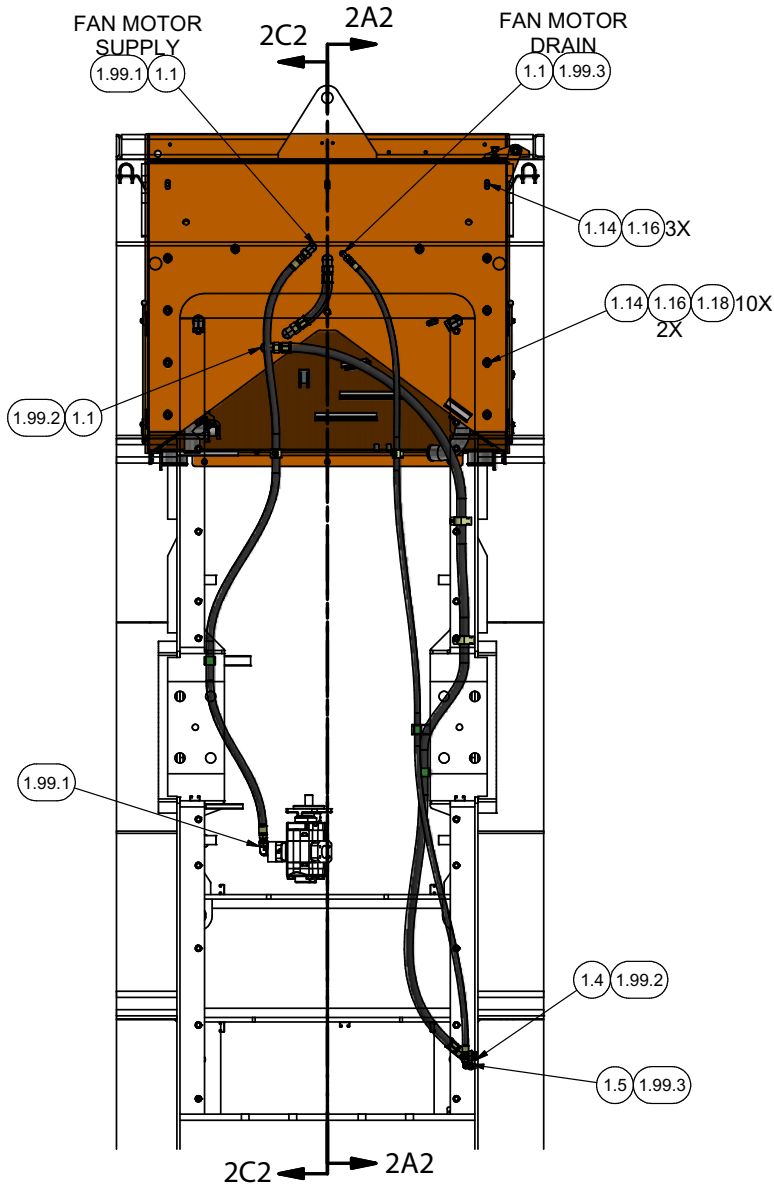
2D2 VIEW FROM BOTTOM
