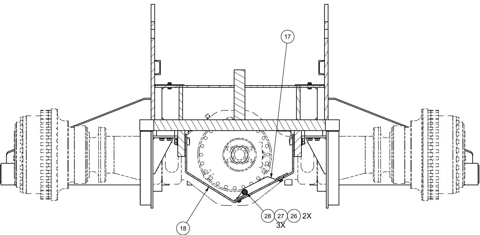
SECTION 3D1-3D1
