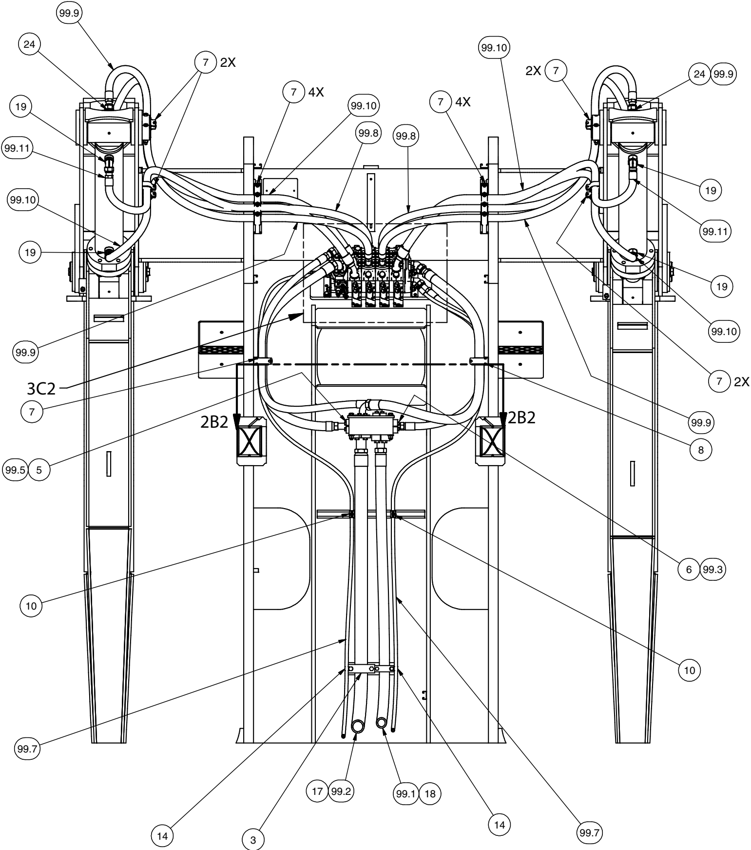
SECTION 2A1-2A1 SOME PARTS REMOVED FOR CLARITY
