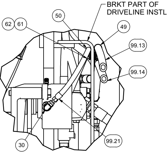
DETAIL 3G3 PARKING BRAKE
