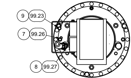
SECTION 3R1-3R1 LH BRAKE HUB PLUMBING SINGLE FRONT TIRES UNIT SHOWN
