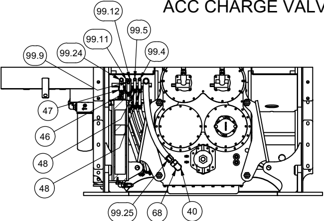
SECTION 3J1-3J1 TRANS SUMP RETURN
