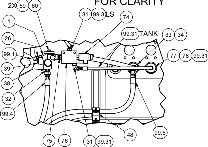
DETAIL 3E3 BRAKE DRAINS SOME PARTS REMOVED FOR CLARITY
