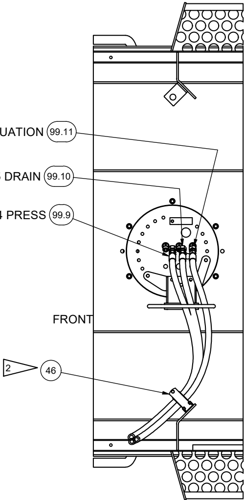
SECTION 2B1-2B1 CAB CONNECTIONS
