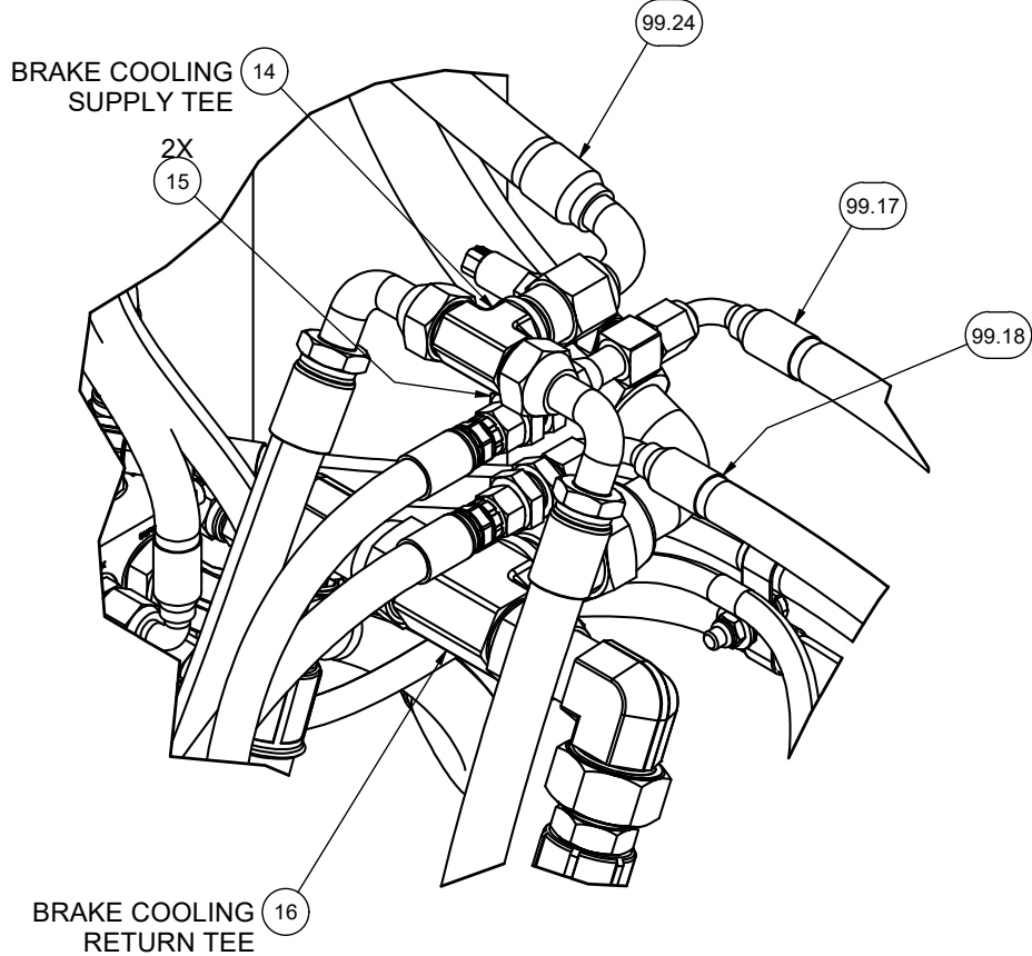
DETAIL 2A2 FRONT AXLE DISTRIBUTION
