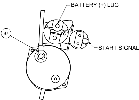
SECTION 2D2-2D2 STARTER WIRING DETAIL ITEMS REMOVED FOR CLARITY
