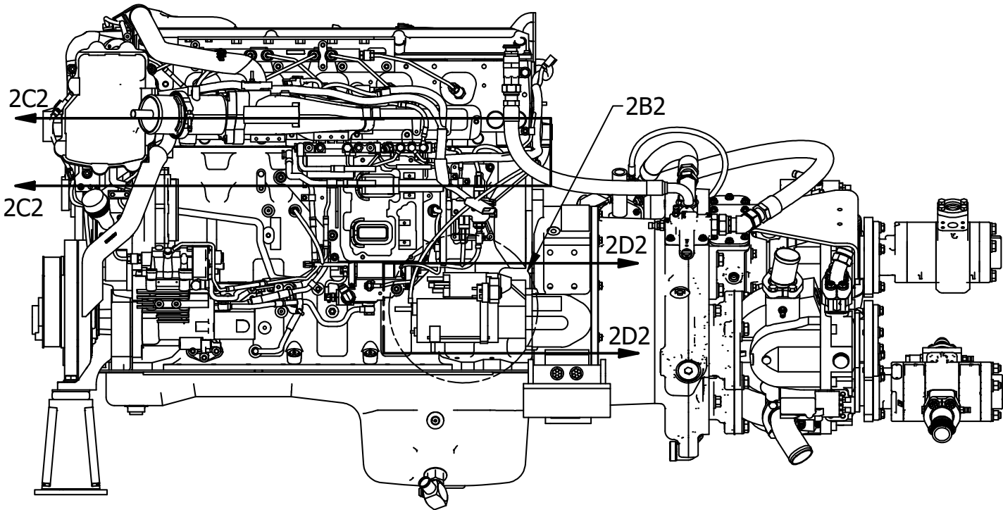
RH SIDE VIEW
