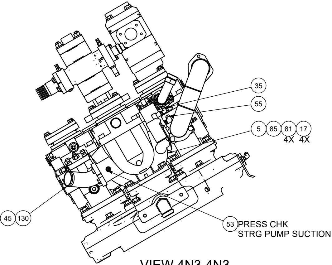
VIEW 4N3-4N3 STRG PUMP FITTING INSTL
