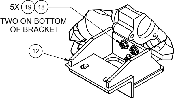
DETAIL 1A1 TYP BOTH SIDES
