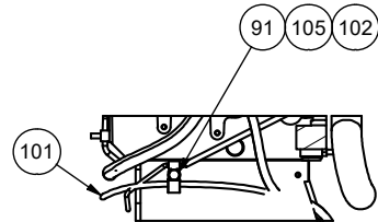
SECTION 2C2-2C2 ITEMS REMOVED FOR CLARITY
