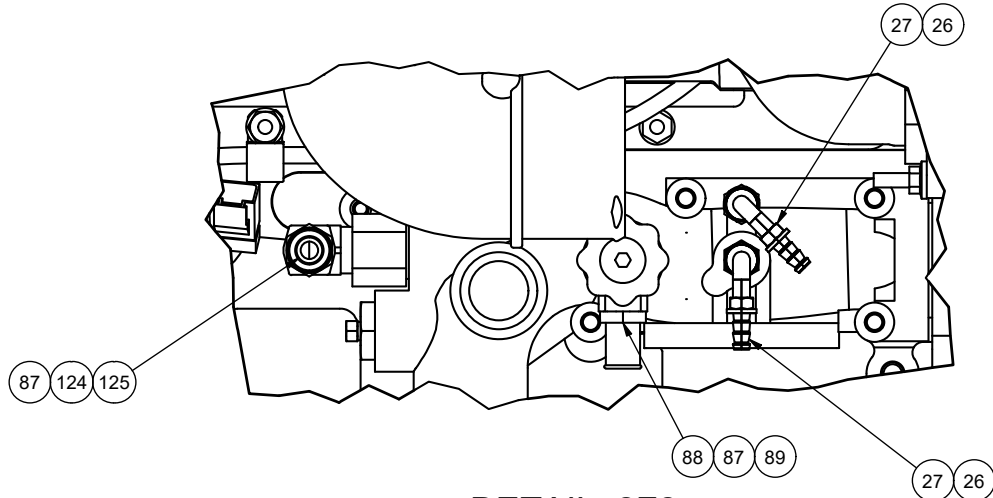
DETAIL 2F2 CAB HEATER COOLANT PORTS
