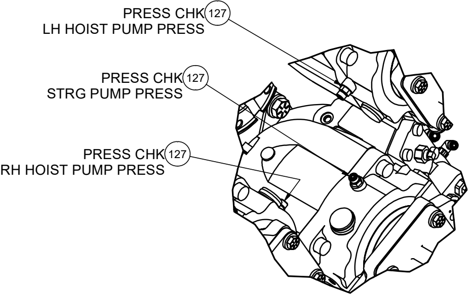
DETAIL 4P4 HOIST PUMP PRESSURE CHECKS SOME PARTS REMOVED FOR CLARITY
