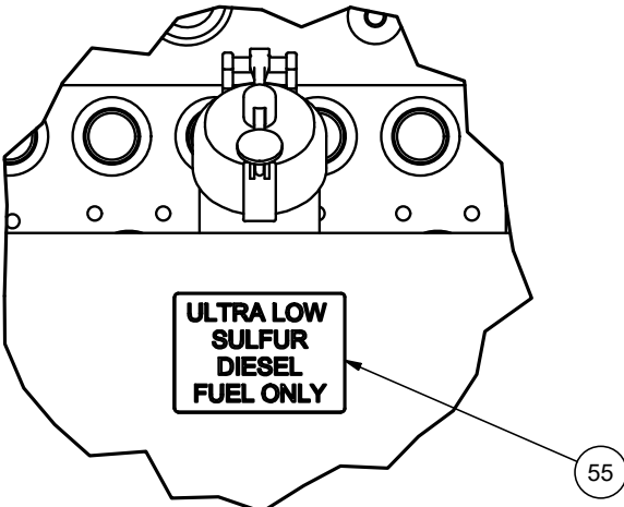
DETAIL 2B2 FUEL FILL
