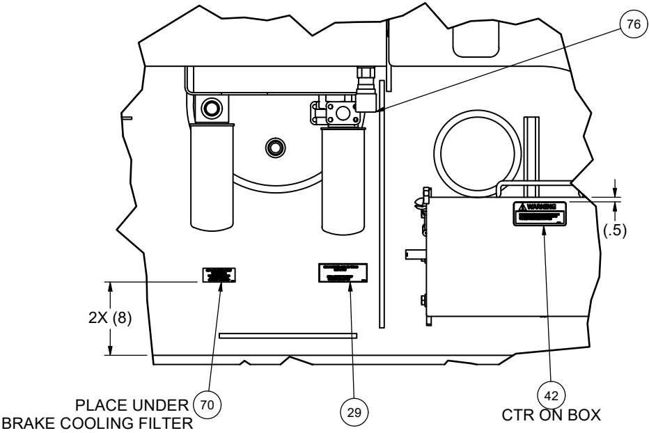
DETAIL 3D3
