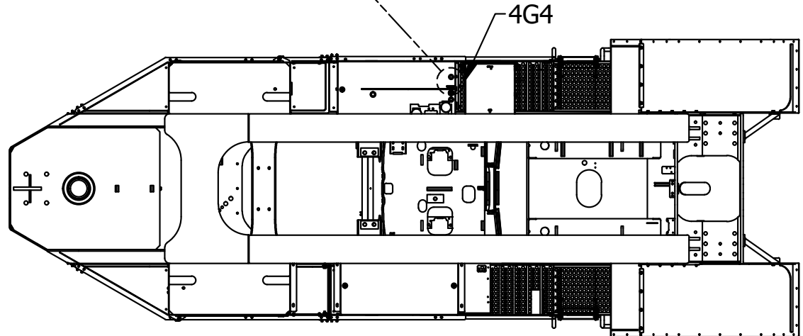
BOTTOM VIEW
