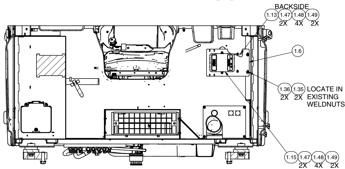
SECTION 3F2-3F2
