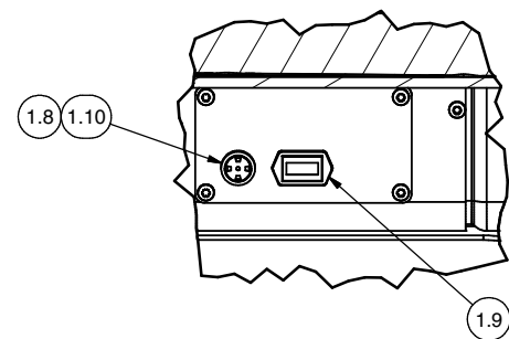
DETAIL 3C3
