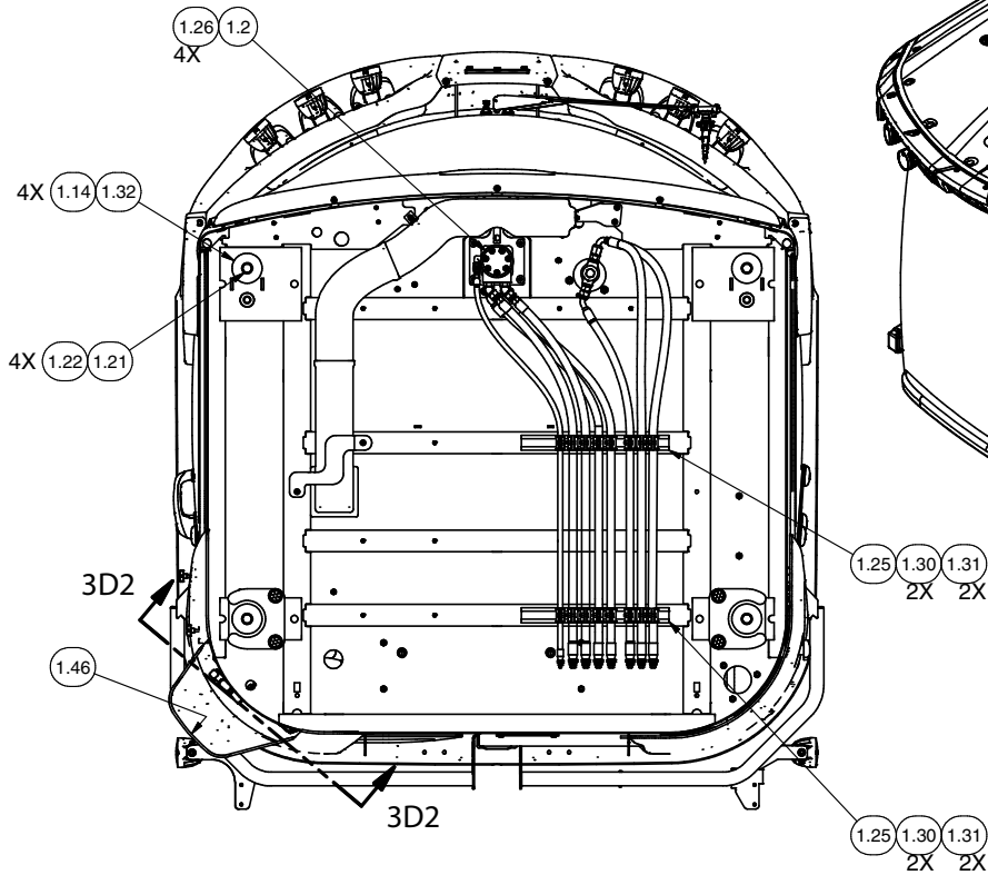
VIEW 2C2-2C2
