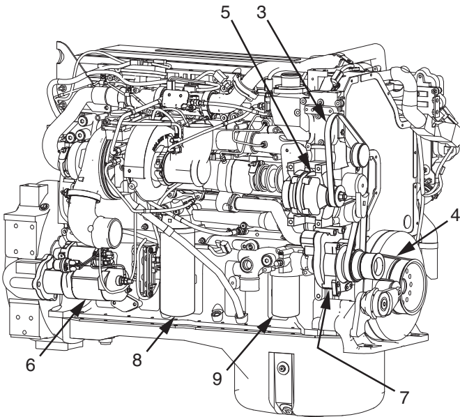
Left Side of Engine
