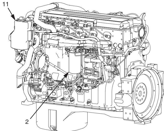
Right Side of Engine
