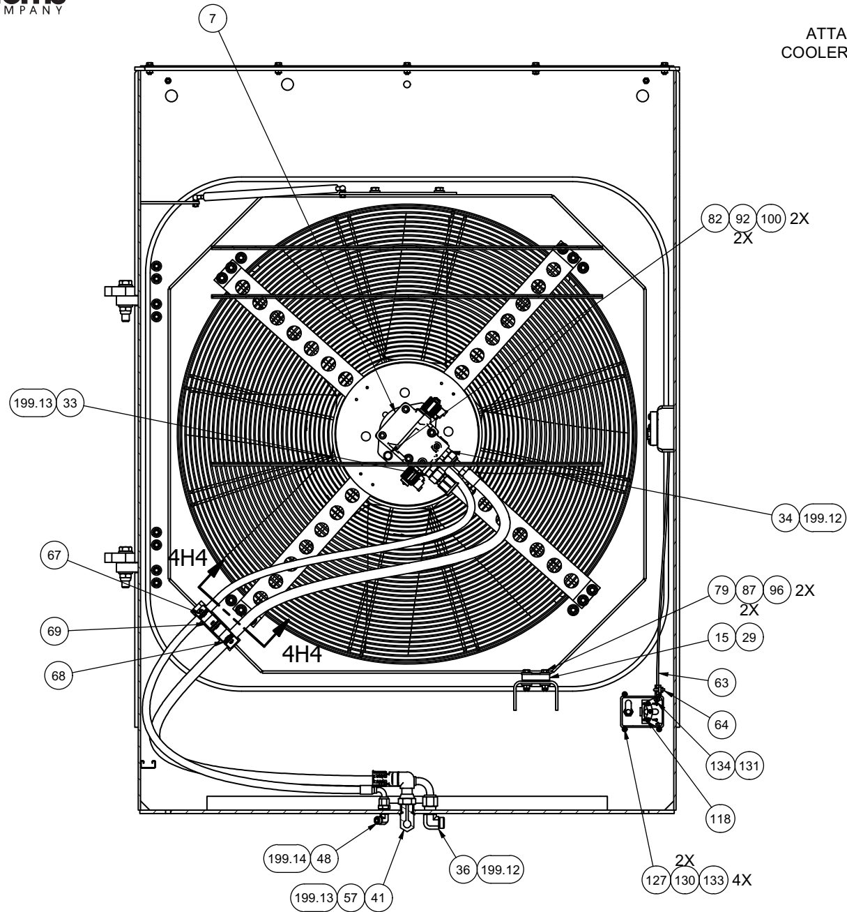
SECTION 4F2-4F2
