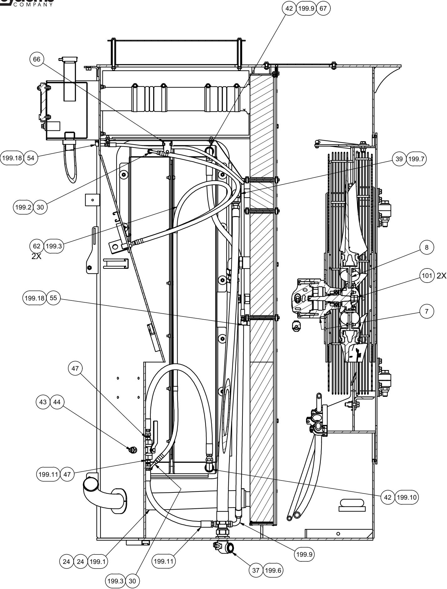
SECTION 6L2-6L2
