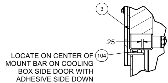
DETAIL 4M4 TYP. BOTH SIDES
