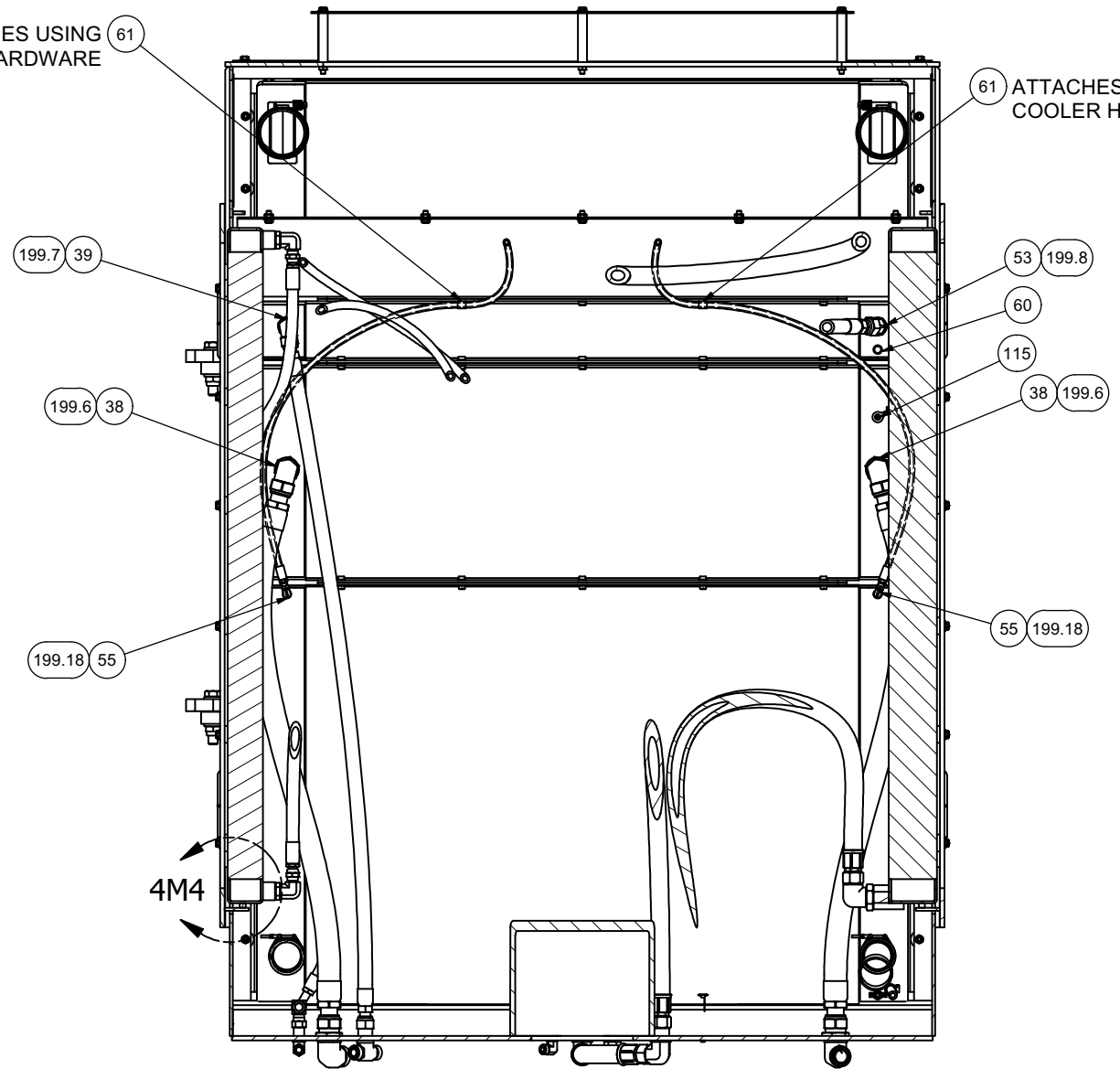
SECTION 4G2-4G2
