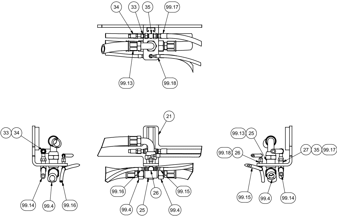
DETAIL 2D2 BRAKE PLUMBING DISTRIBUTION BRKT
