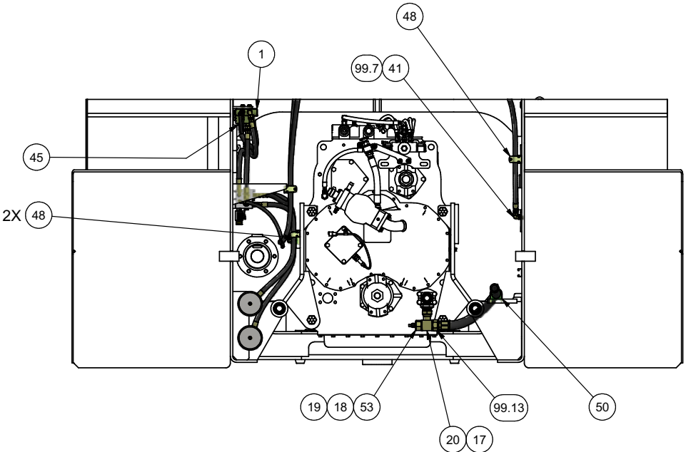
SECTION 3H1-3H1 BRAKE COOLING TRANS SUMP RETURN
