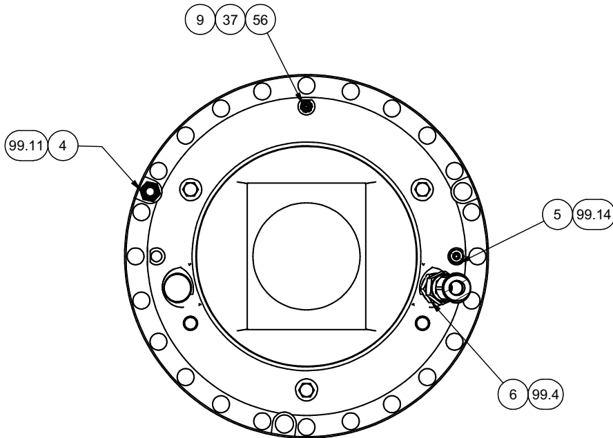
SECTION 2C2-2C2 LH BRAKE HUB PLUMBING
