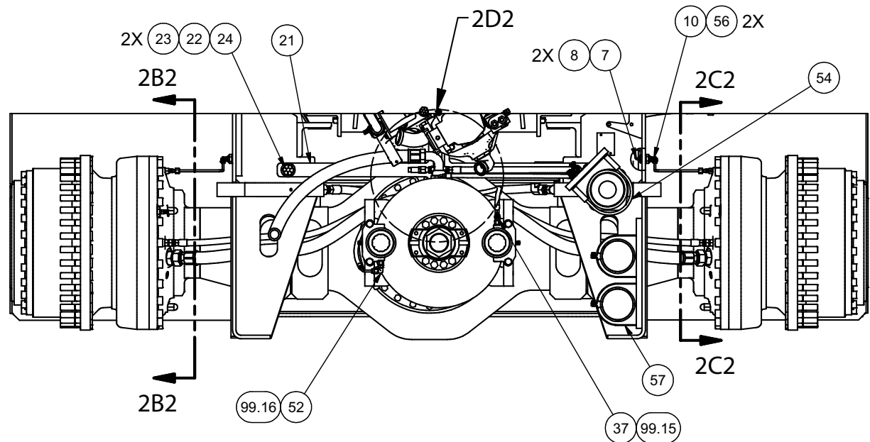
SECTION 2A1-2A1 AXLE PLUMBING
