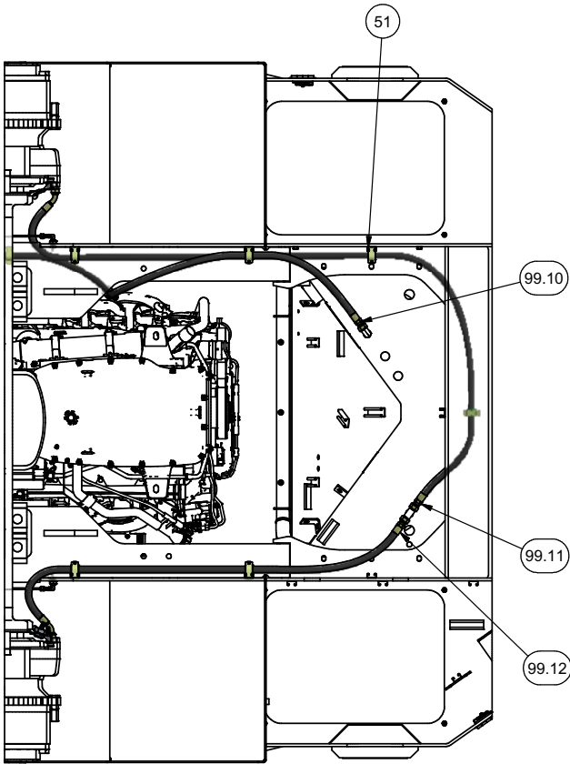
SECTION 3J1-3J1 BRAKE COOLING SUPPLY TO HUBS
