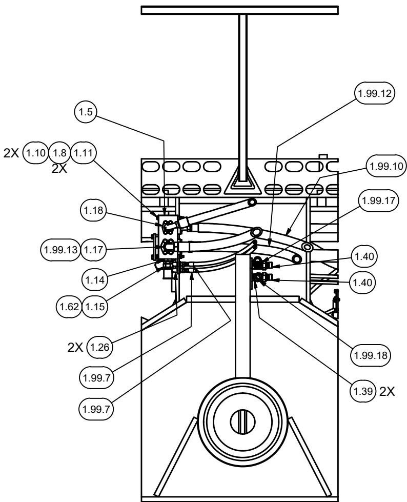
SECTION 3L3-3L3 VIEW ROTATED FOR CLARITY SWIVEL MANIFOLD
