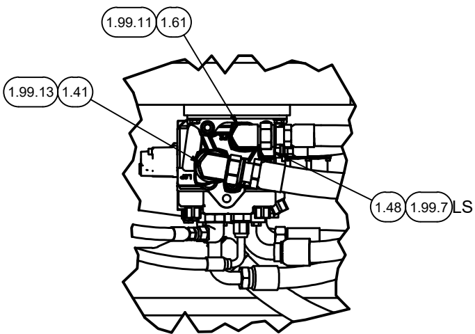
DETAIL 3C3
