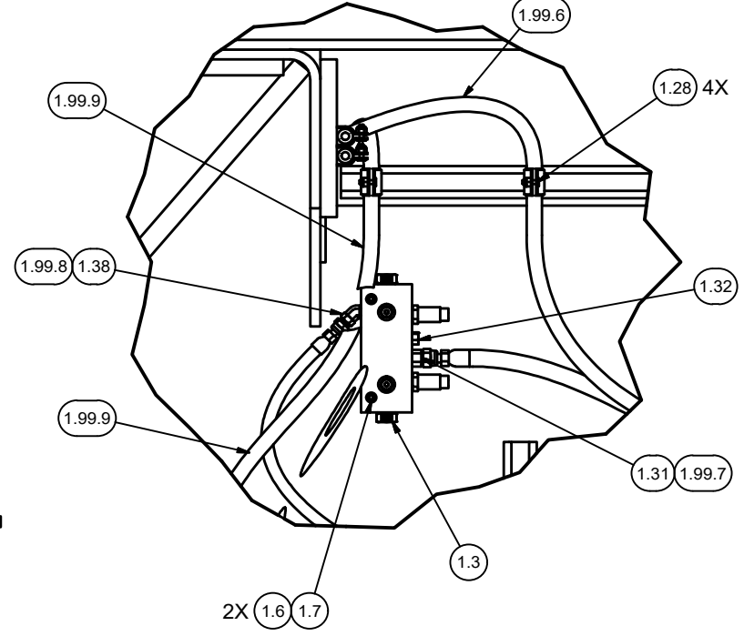
SECTION 4AH4-4AH4 CHECK VALVE ORIENTATION
