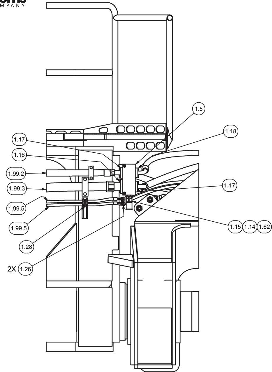
SECTION 5K3-5K3 SWIVEL MANIFOLD PLUMBING
