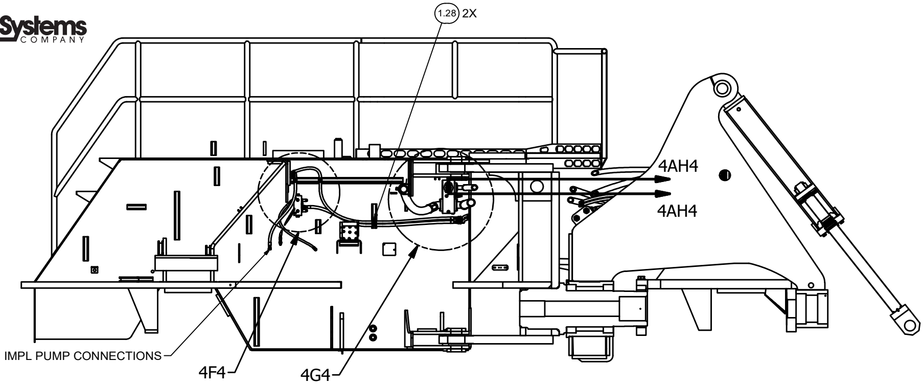
SECTION 4D2-4D2
