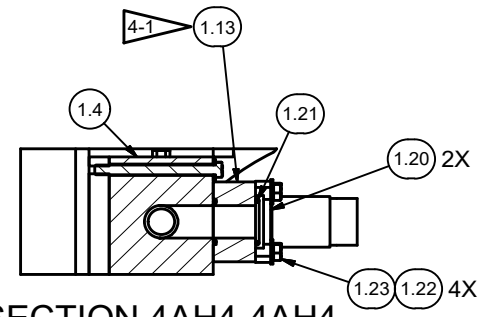
SECTION 4AH4-4AH4 CHECK VALVE ORIENTATION
