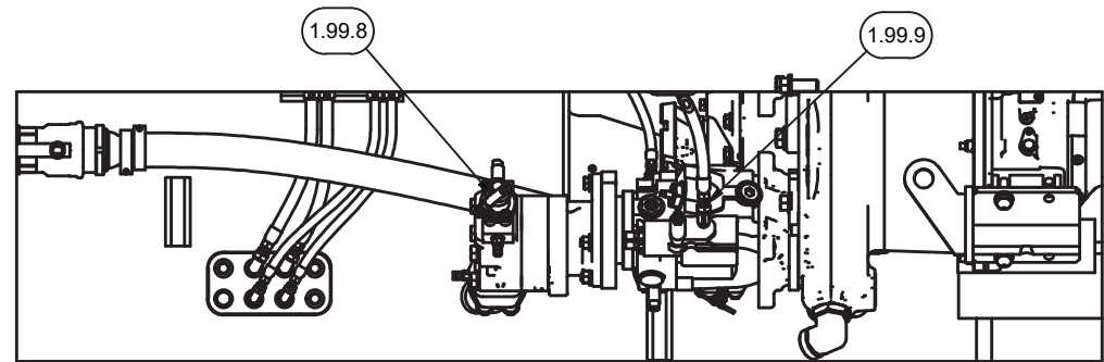
SECTION 5J5-5J5 VIEW CROPED FOR CLARITY IMPLEMENT PUMP CONNECTIONS
