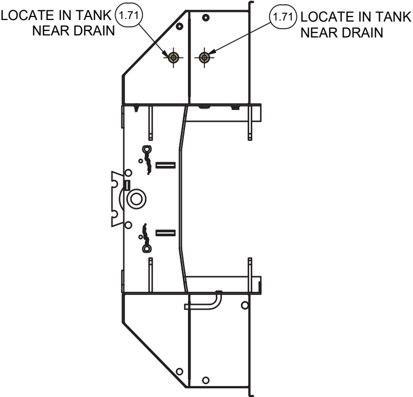
SECTION 2W2-2W2
