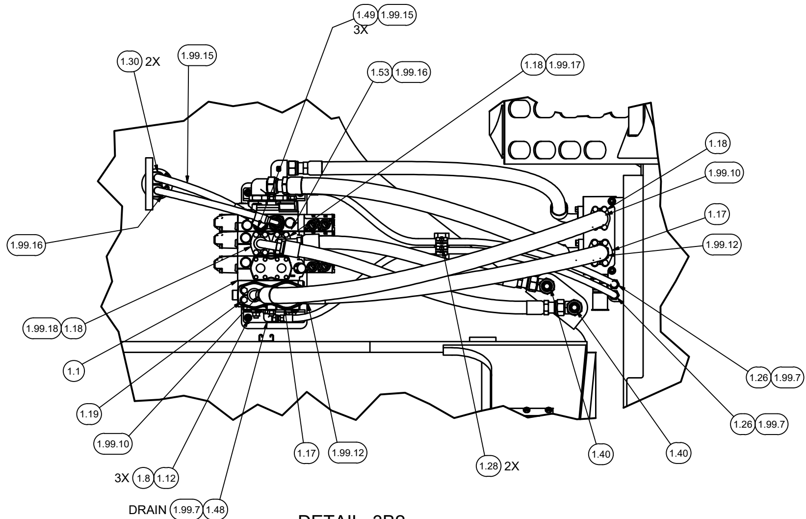
DETAIL 3B2 IMPLEMENT VALVE
