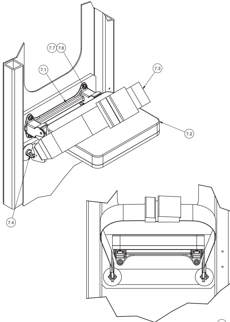
DETAIL 11U11
