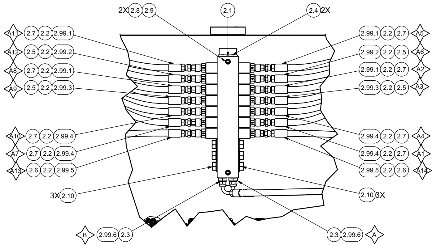
DETAIL 4H2 CARRIAGE DISTRIBUTION BLOCK
