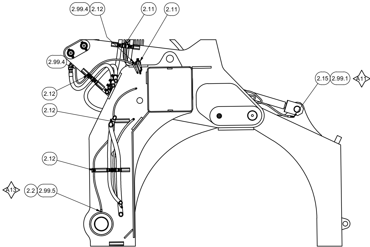
SECTION 4F2-4F2 LH LINE ROUTING
