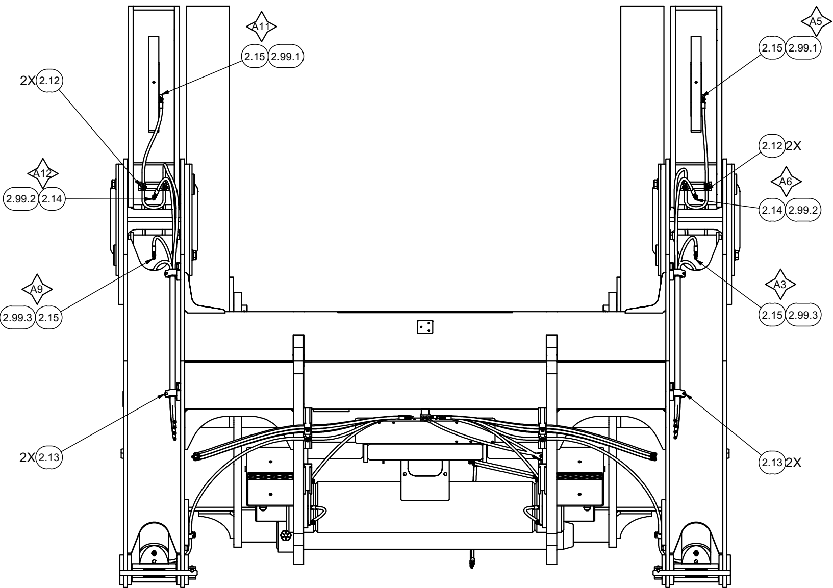
SECTION 3A2-3A2 SOME PARTS HIDDEN FOR CLARITY
