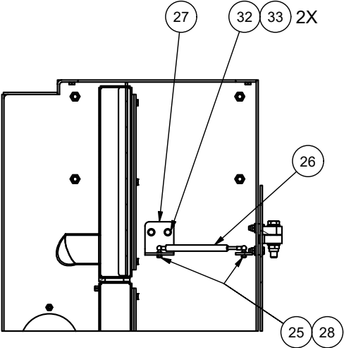
SECTION 1B1-1B1
