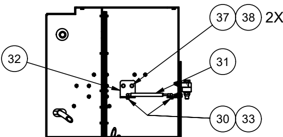
SECTION 1B1-1B1
