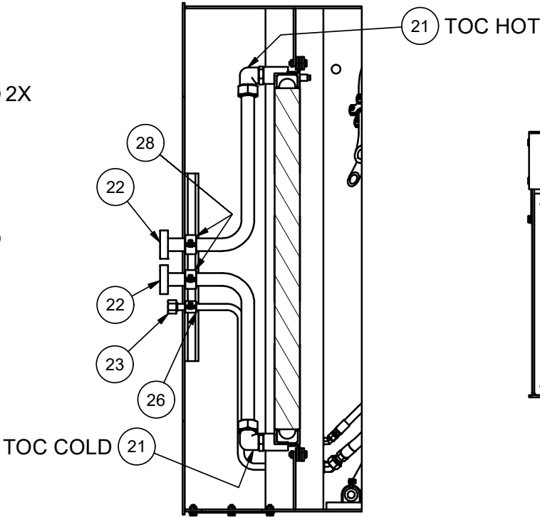
SECTION 1A1-1A1
