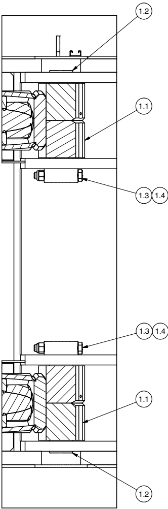
SECTION B-B HOIST CYL BASE RETENTION
