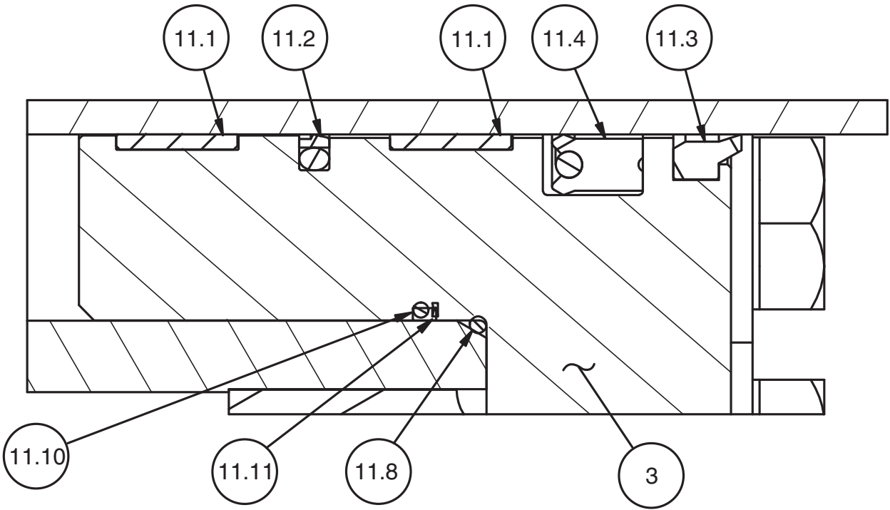
GLAND PACKING DETAIL BARREL/GLAND SEAL USE 11.10 AND 11.11 OR 11.8 NOT BOTH
