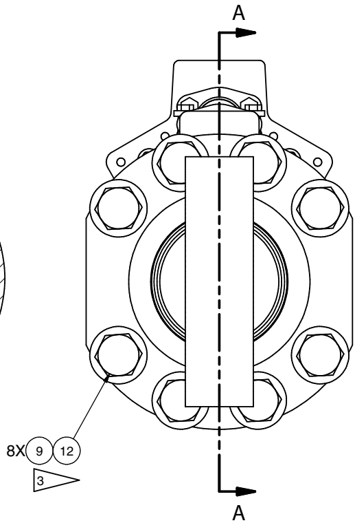
DETAIL C GLAND PACKING BARREL/ GLAND SEAL USE 10.10 AND 10.11 OR 10.2 NOT BOTH
