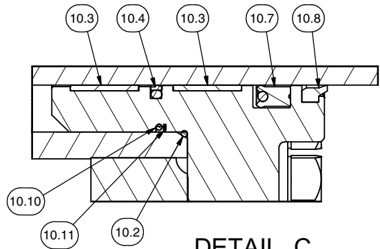
DETAIL C GLAND PACKING BARREL/ GLAND SEAL USE 10.10 AND 10.11 OR 10.2 NOT BOTH
