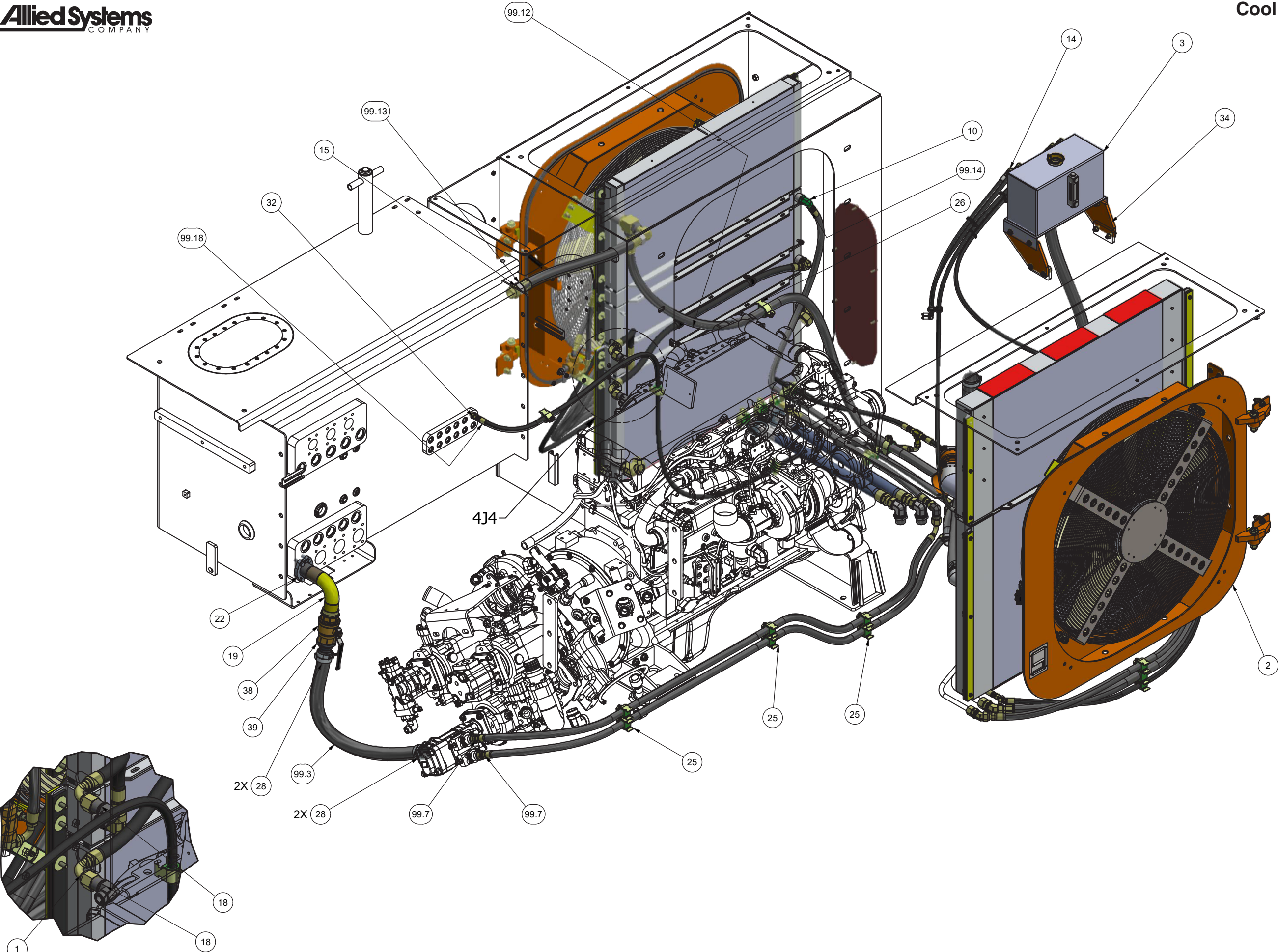
DETAIL 4J4
