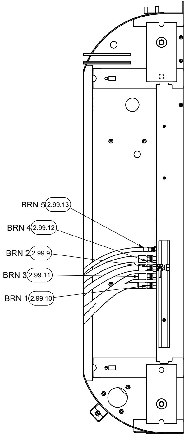
SECTION 7P6-7P6 ORBITROL STEERING LINES
