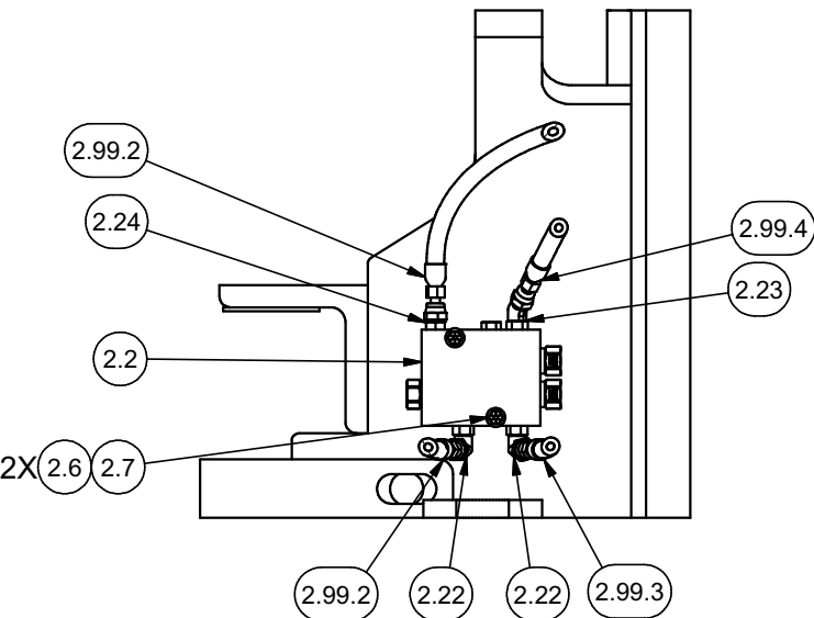
SECTION 6M6-6M6 STRG LS PRIORITY MANIFOLD
