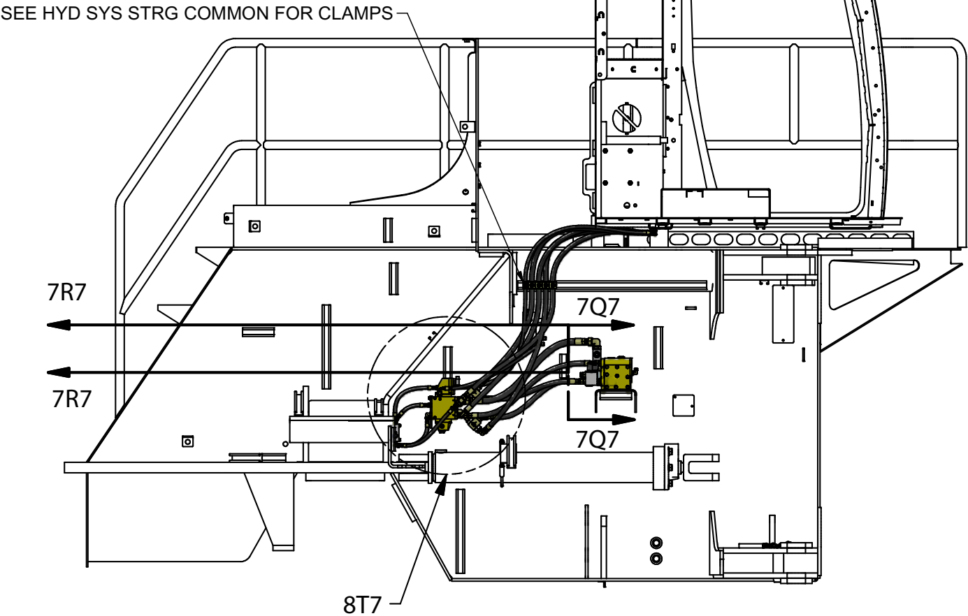
SECTION 7N6-7N6
