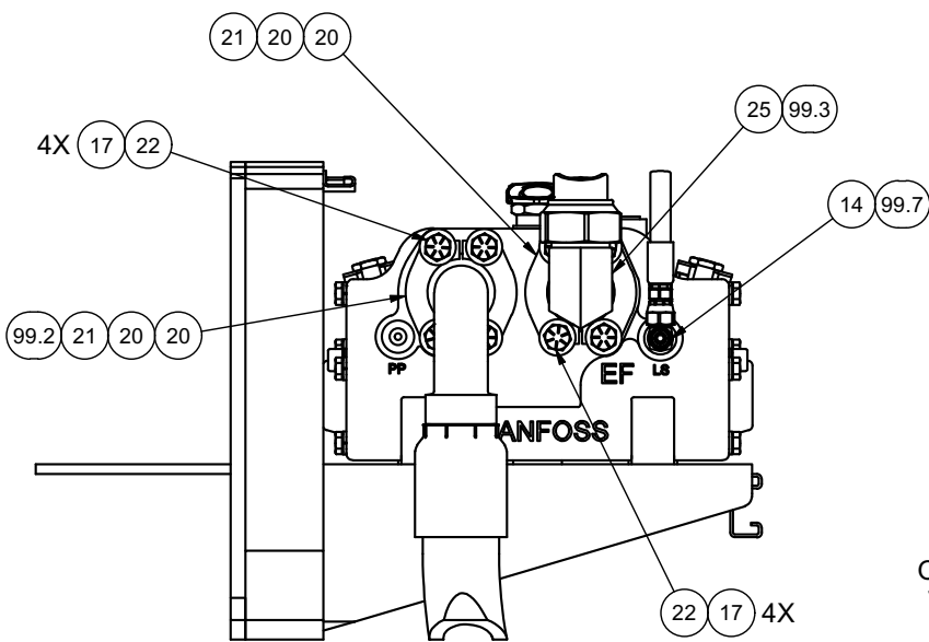
SECTION 11Q10-11Q10 POWER UNIT REMOVED FOR CLARITY
