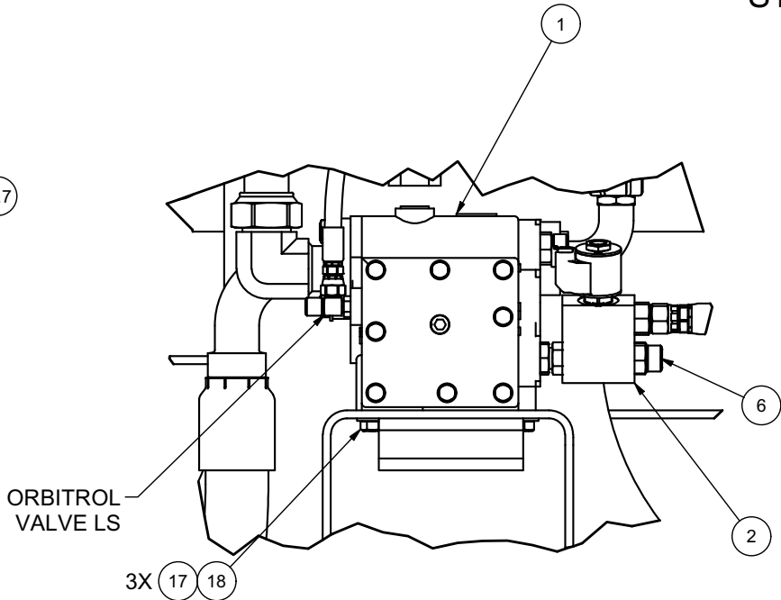
DETAIL 11T11 STEERING FLOW AMP
