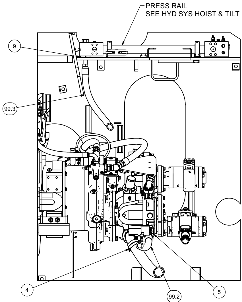
SECTION 11R10-11R10 STRG PUMP CONNECTIONS
