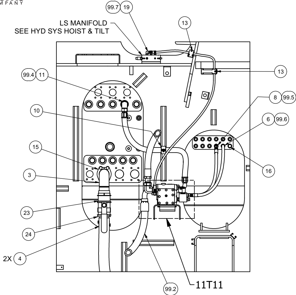
SECTION 11Q10-11Q10 POWER UNIT REMOVED FOR CLARITY
