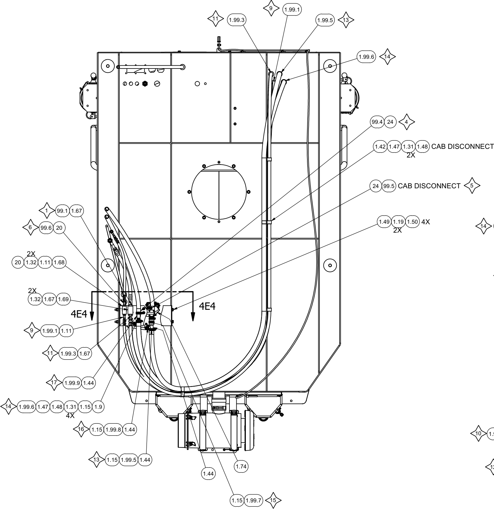
SECTION 4F2-4F2
