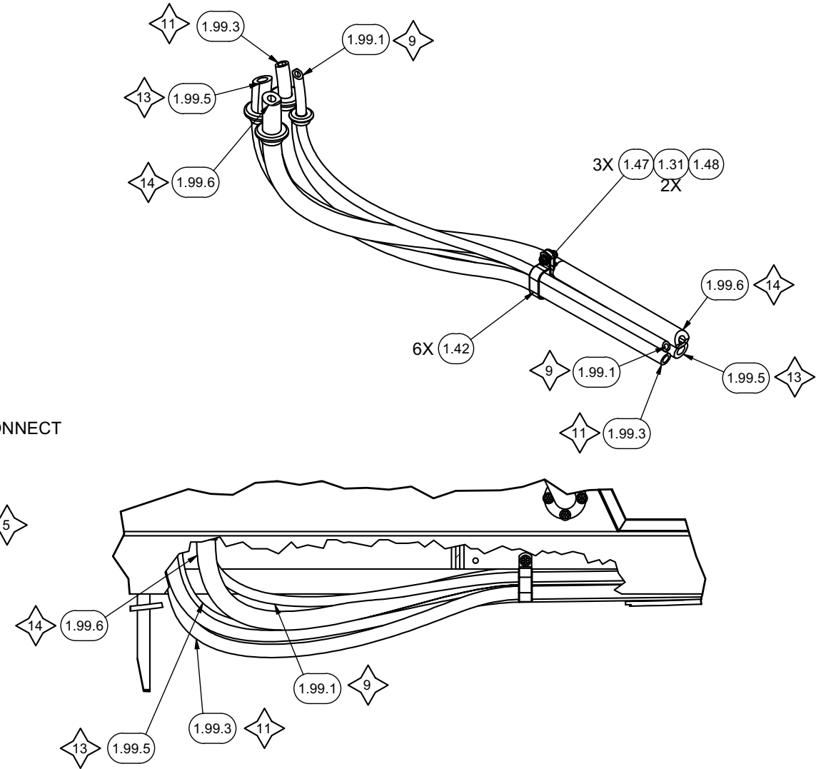
DETAIL 4G2 AC/HEATER ROUTING DETAIL
