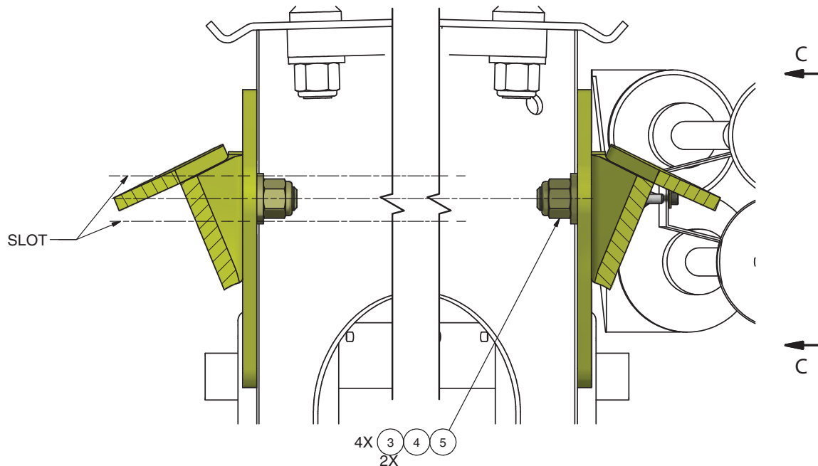
SECTION B-B
