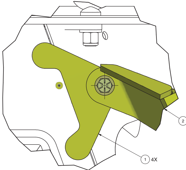
DETAIL A
