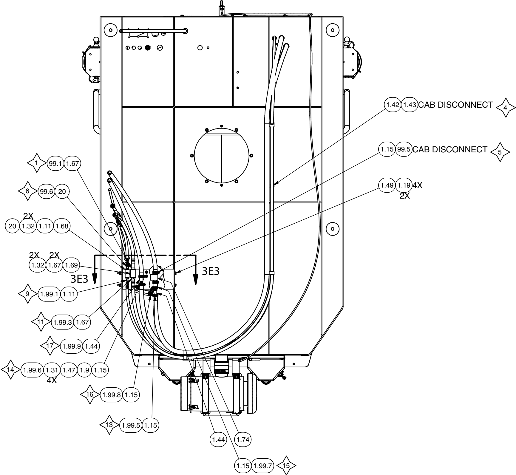
SECTION 3F2-3F2
