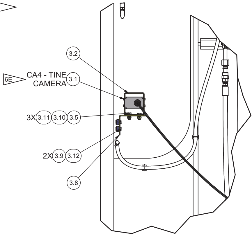
DETAIL 4Q4 TINE CAMERA
