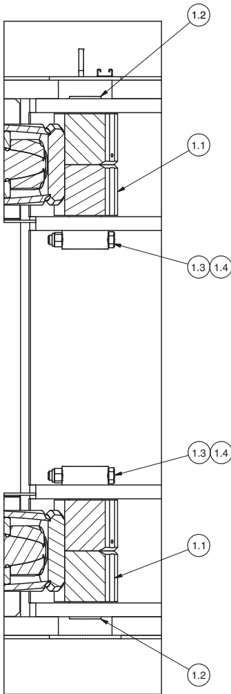
SECTION B-B HOIST CYL BASE RETENTION
