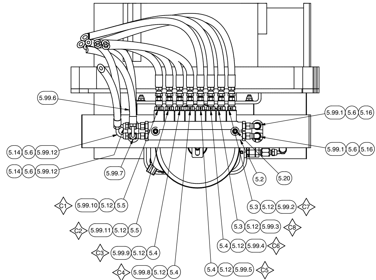
VIEW 12V10-12V10 CHASSIS GREASE DISTRIBUTION MANIFOLD
