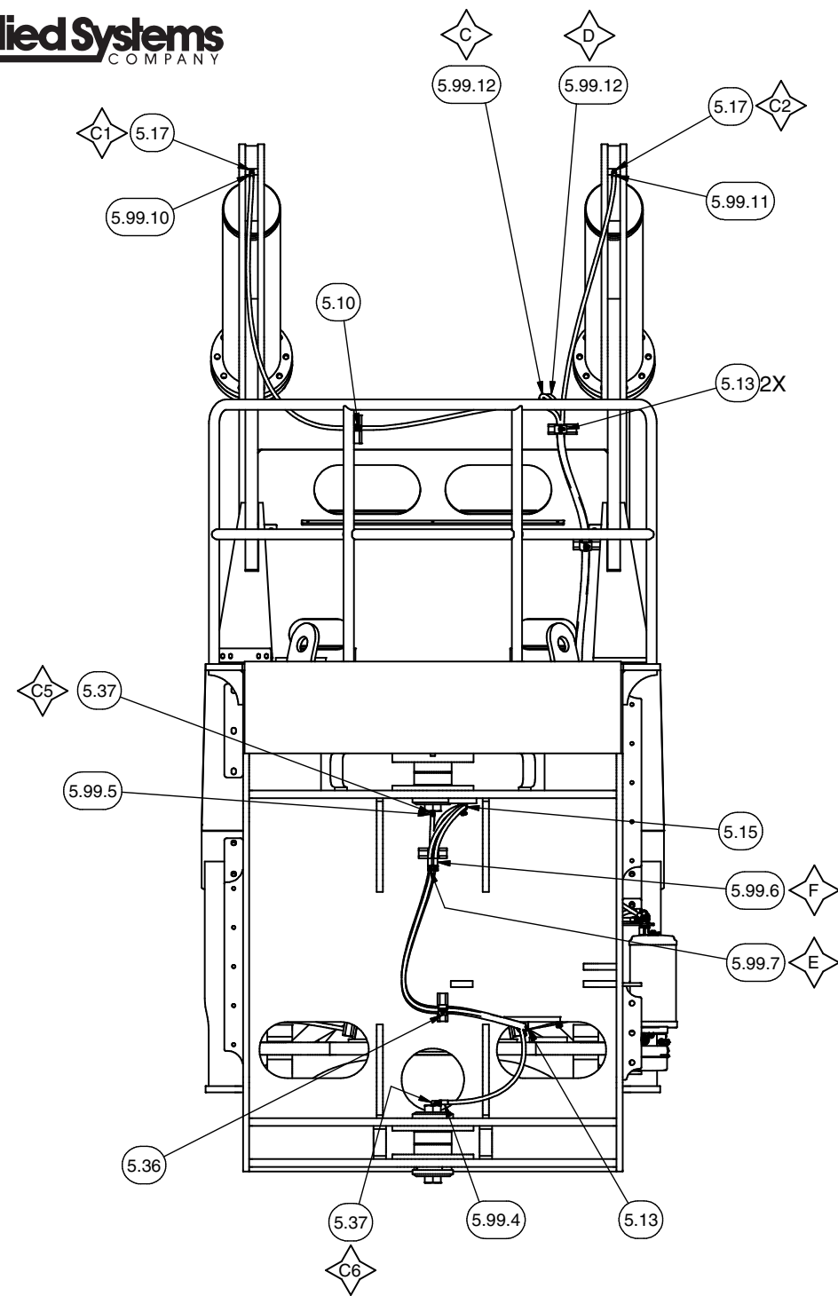
REAR VIEW
