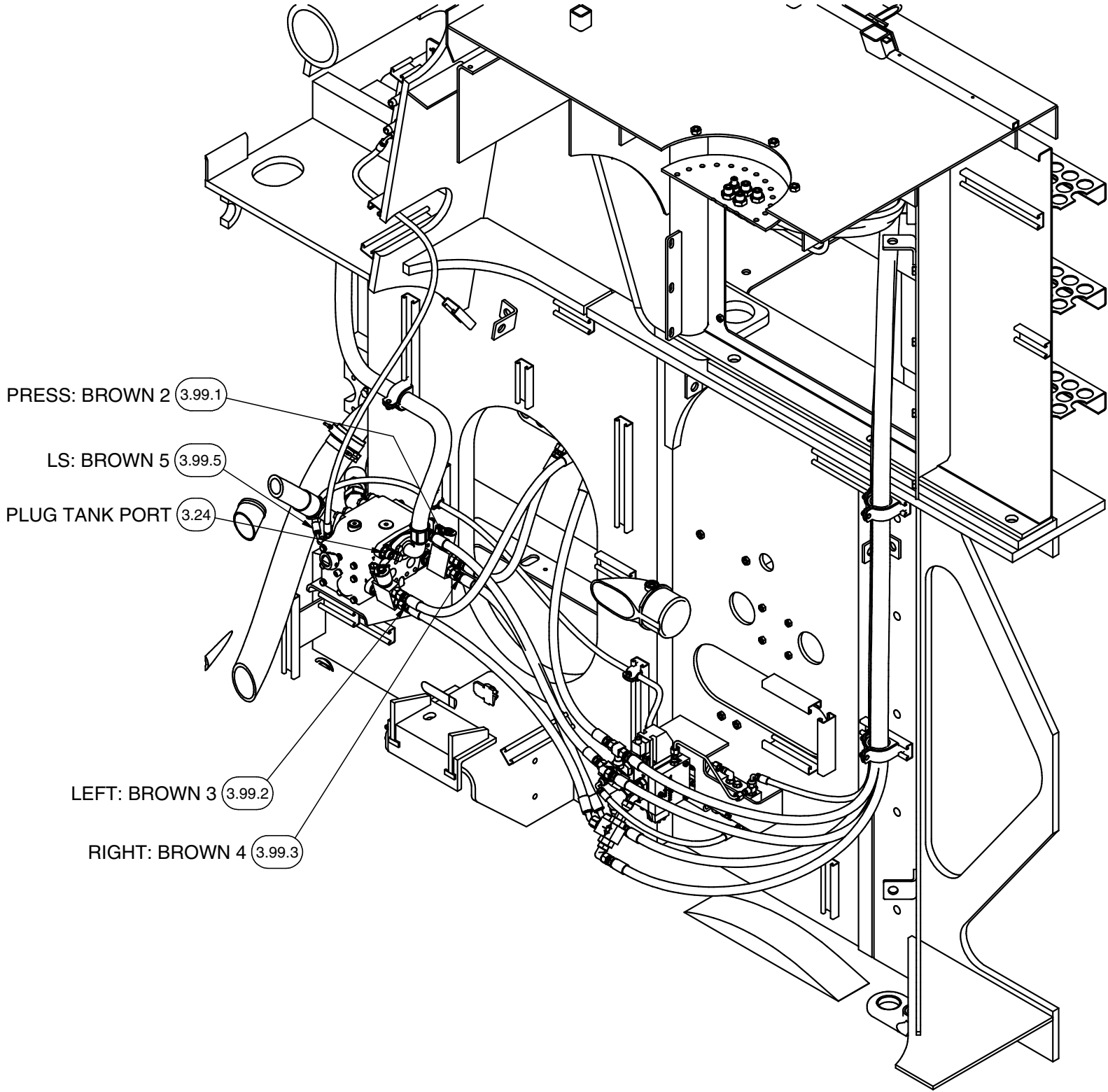
ISO PROJECTION OF VIEW 7J6
