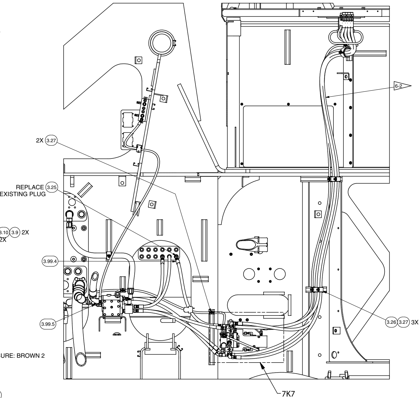
SECTION 7J6-7J6 JOYSTICK STEERING INSTALL SOME PARTS REMOVED FOR CLARITY
