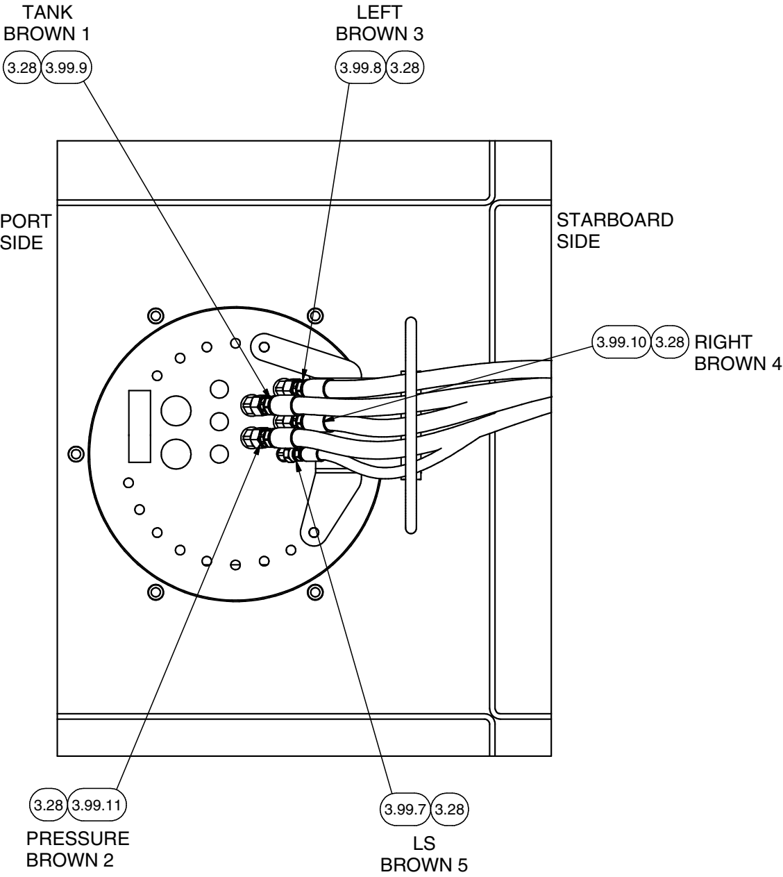
SECTION 8L6-8L6 SEAT SWIEVL BULKHEAD PLATE
