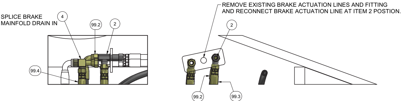
DETAIL B LH CYLINDER POCKET PLATE REMOVED FOR CLARITY
