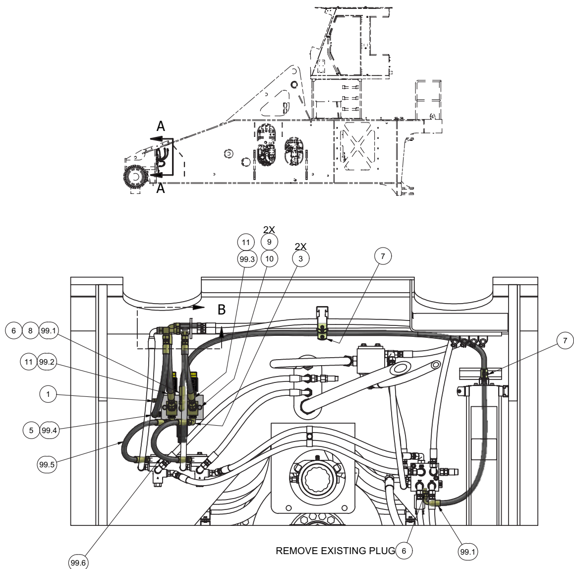
SECTION A-A LH HOIST CYLINDER POCKET PLATE REMOVED FOR CLARITY
