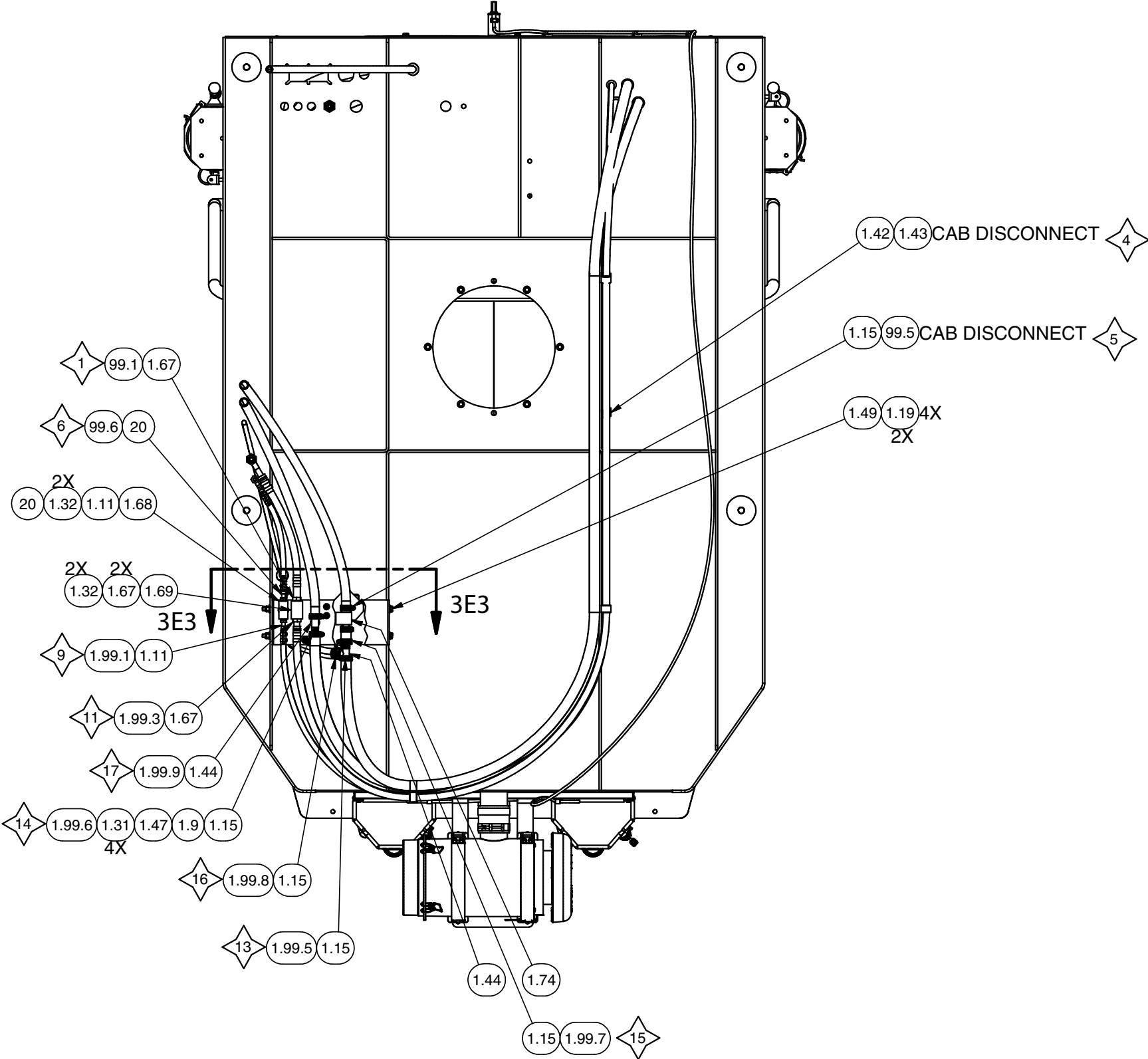
SECTION 3F2-3F2
