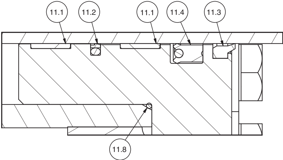
GLAND PACKING DETAIL
