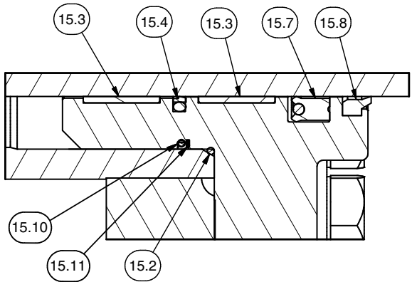
DETAIL B GLAND PACKING BARREL / GLAND SEAL USE 15.10 AND 15.11 OR 15.2 NOT BOTH
