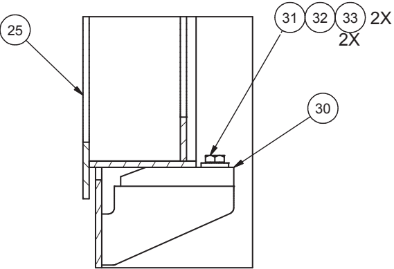
SECTION 4N4-4N4
