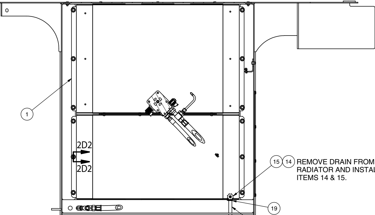
SECTION 2C1-2C1
