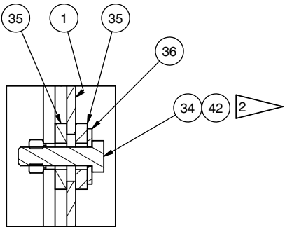
SECTION 2D2-2D2 INSTL TYP FOR ITEMS 34-36 (12 PLACES)
