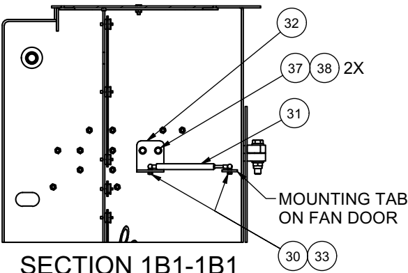
SECTION 1B1-1B1
