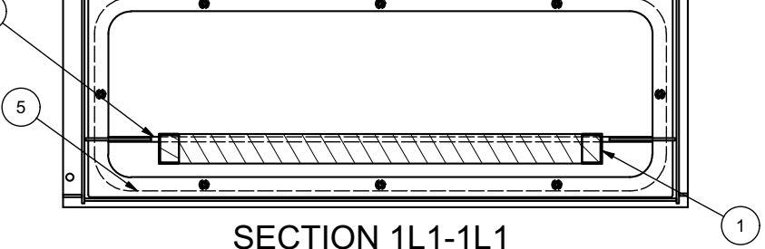
SECTION 1L1-1L1
